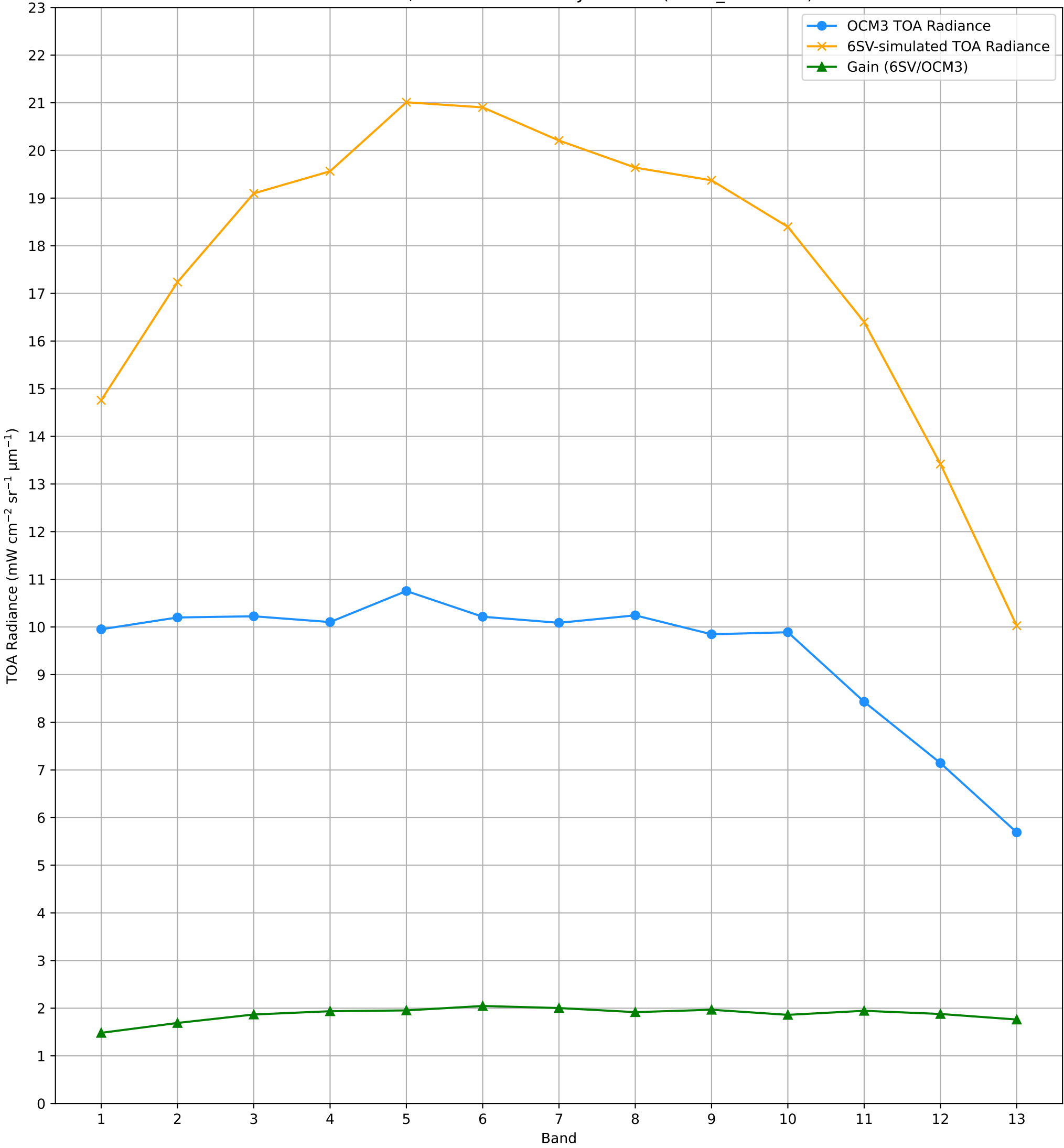
TOA Radiance (OCM3 vs. 6SV) over RVUS RadCalNet Site Lat: 38.497°, Lon: -115.69° - 17-JUN-2025 (STRIP_ID: 13516)
