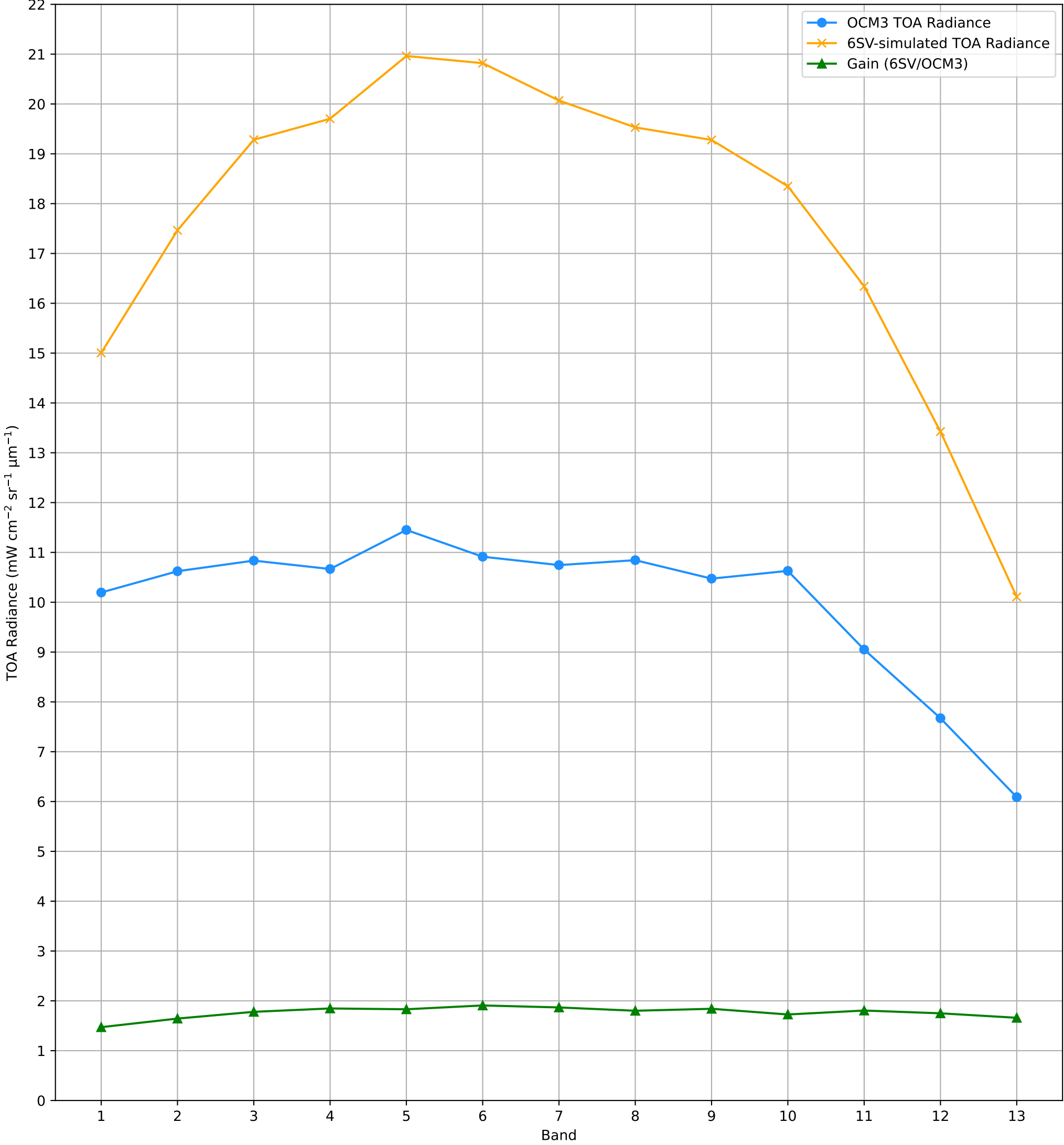
TOA Radiance (OCM3 vs. 6SV) over RVUS RadCalNet Site Lat: 38.497°, Lon: -115.69° - 15-JUN-2025 (STRIP_ID: 13487)
