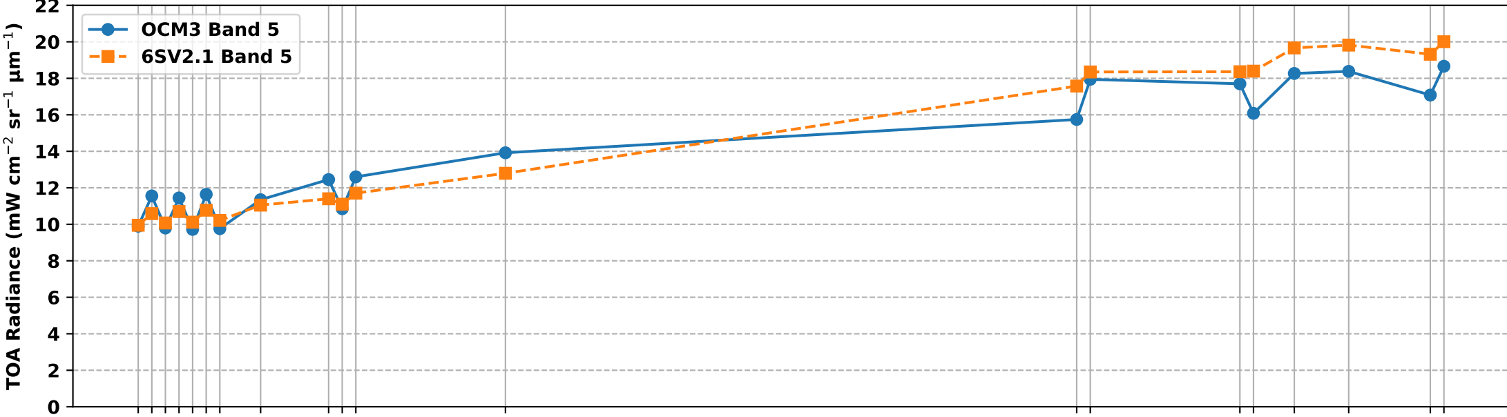
OCM3 Band 5 vs 6S Simulated Band 5 TOA Radiance over RVUS RadCalNet Site (Jan-Apr 2025)
