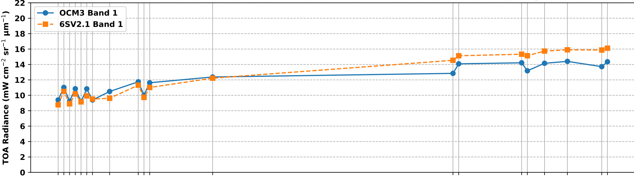
OCM3 Band 1 vs 6S Simulated Band 1 TOA Radiance over RVUS RadCalNet Site (Jan-Apr 2025)
