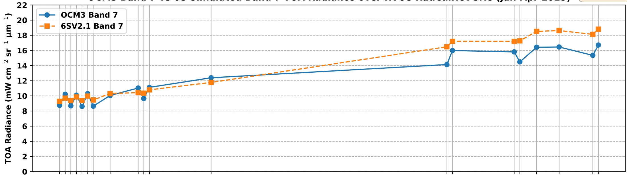
OCM3 Band 7 vs 6S Simulated Band 7 TOA Radiance over RVUS RadCalNet Site (Jan-Apr 2025)
