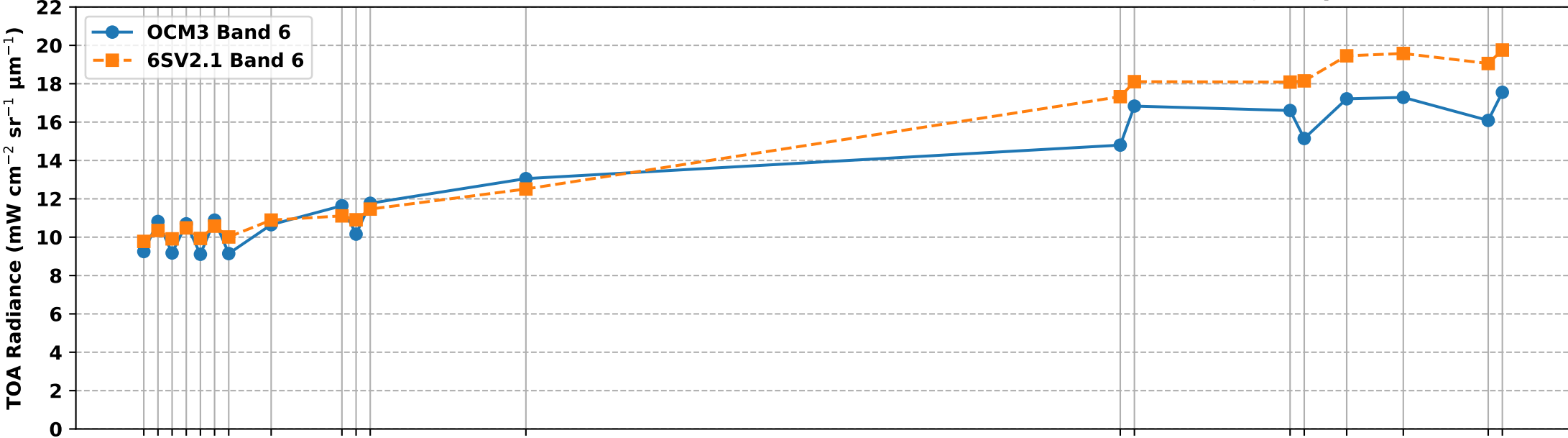
OCM3 Band 6 vs 6S Simulated Band 6 TOA Radiance over RVUS RadCalNet Site (Jan-Apr 2025)
