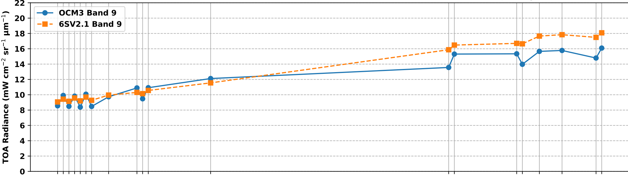
OCM3 Band 9 vs 6S Simulated Band 9 TOA Radiance over RVUS RadCalNet Site (Jan-Apr 2025)
