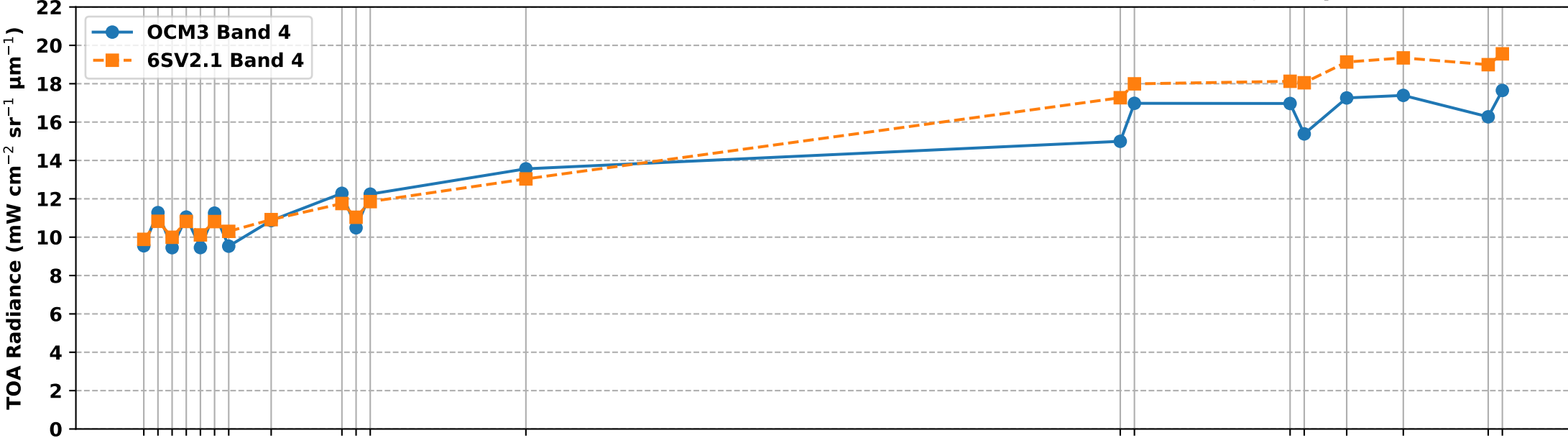
OCM3 Band 4 vs 6S Simulated Band 4 TOA Radiance over RVUS RadCalNet Site (Jan-Apr 2025)
