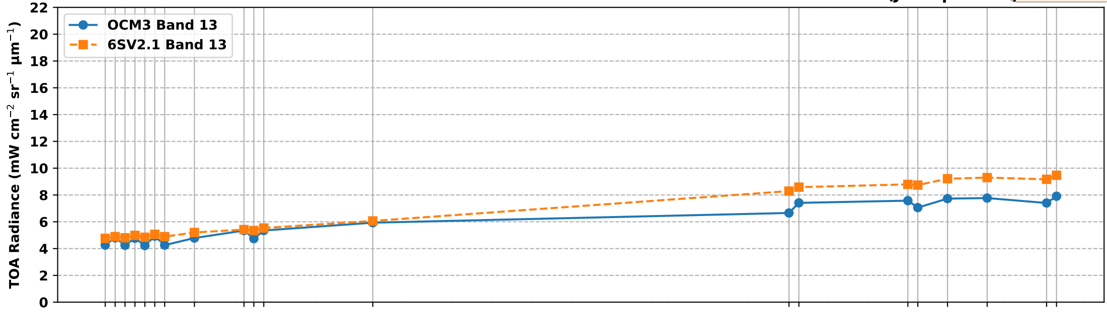
OCM3 Band 13 vs 6S Simulated Band 13 TOA Radiance over RVUS RadCalNet Site (Jan-Apr 2025)
