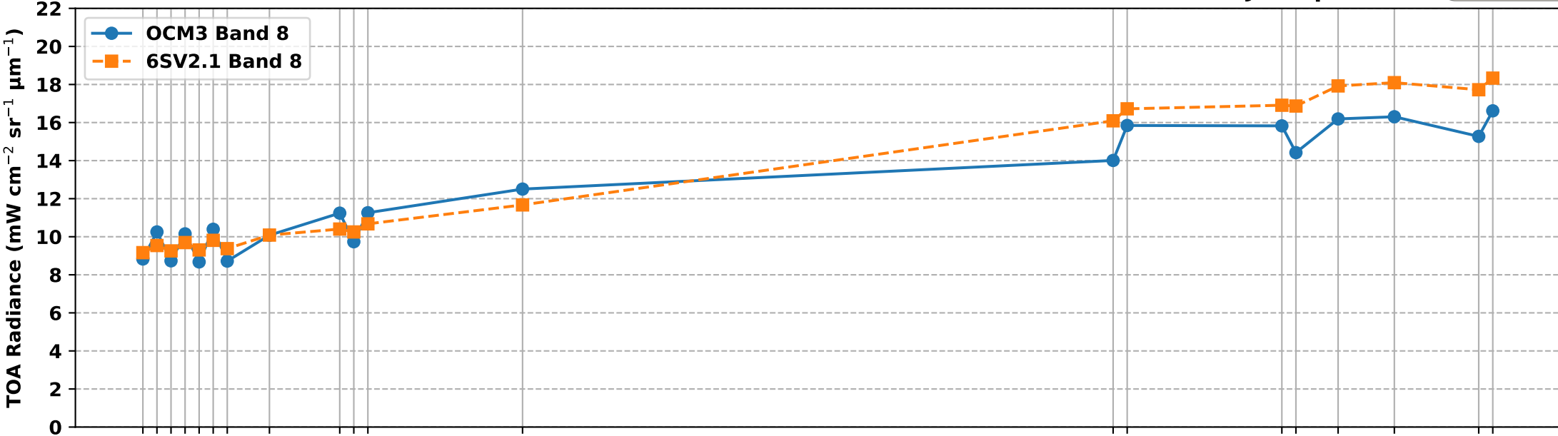
OCM3 Band 8 vs 6S Simulated Band 8 TOA Radiance over RVUS RadCalNet Site (Jan-Apr 2025)
