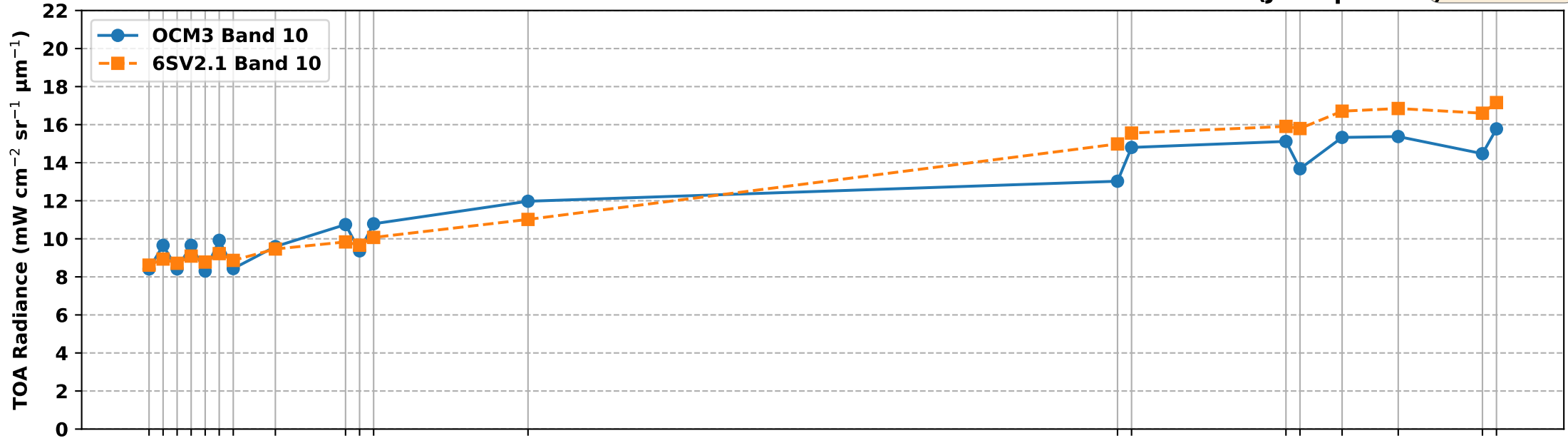
OCM3 Band 10 vs 6S Simulated Band 10 TOA Radiance over RVUS RadCalNet Site (Jan-Apr 2025)
