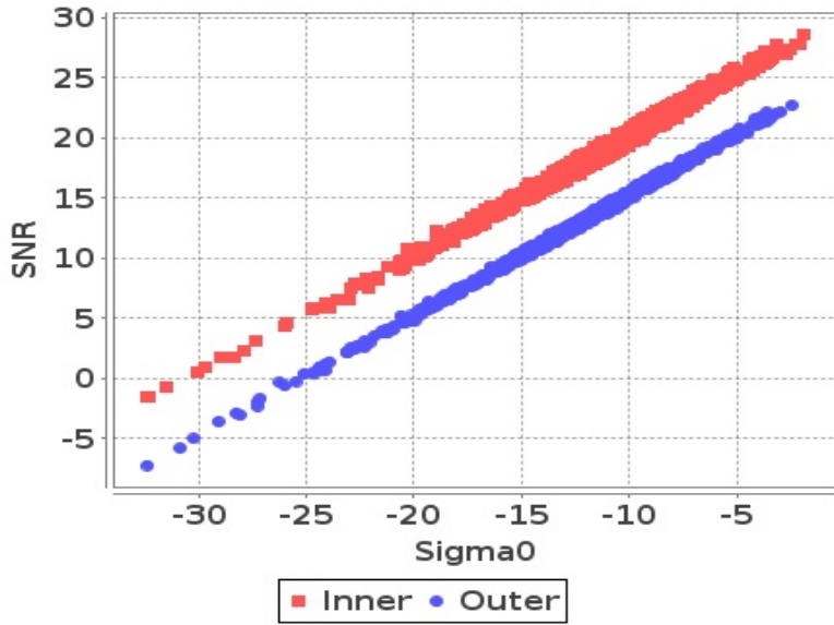
Slice-Land
