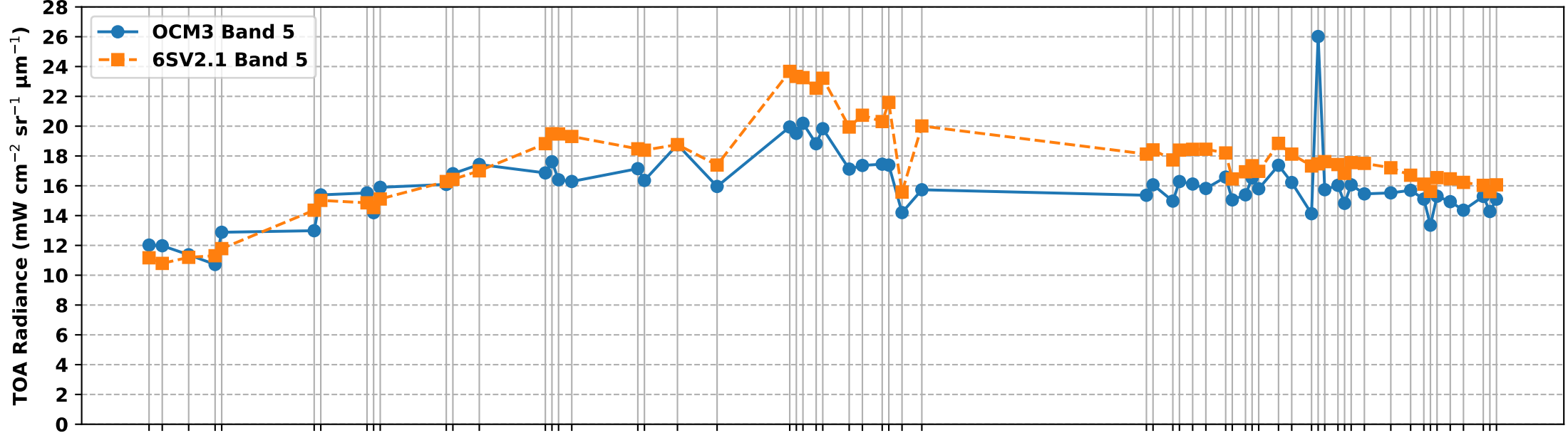
OCM3 Band 5 vs 6S Simulated Band 5 TOA Radiance over RVUS RadCalNet Site (Feb-Aug 2026)
