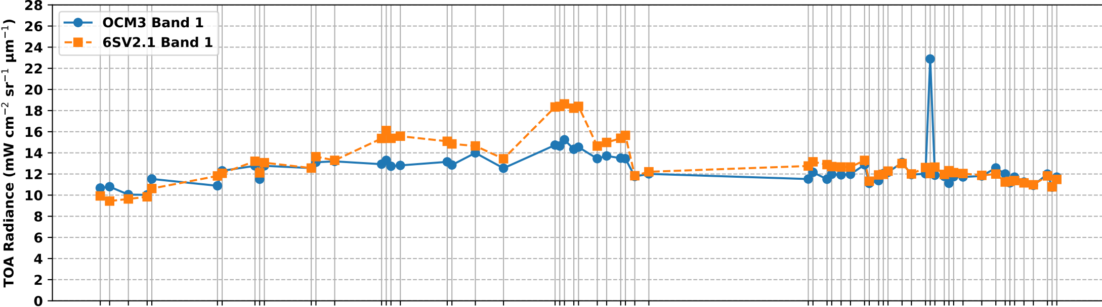
OCM3 Band 1 vs 6S Simulated Band 1 TOA Radiance over RVUS RadCalNet Site (Feb-Aug 2026)
