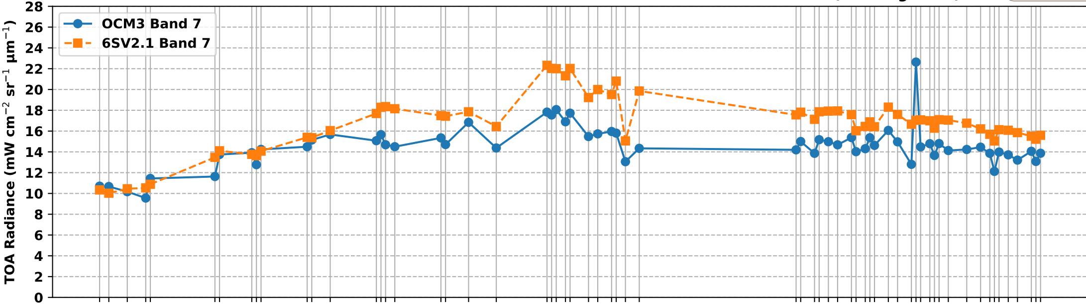
OCM3 Band 7 vs 6S Simulated Band 7 TOA Radiance over RVUS RadCalNet Site (Feb-Aug 2026)
