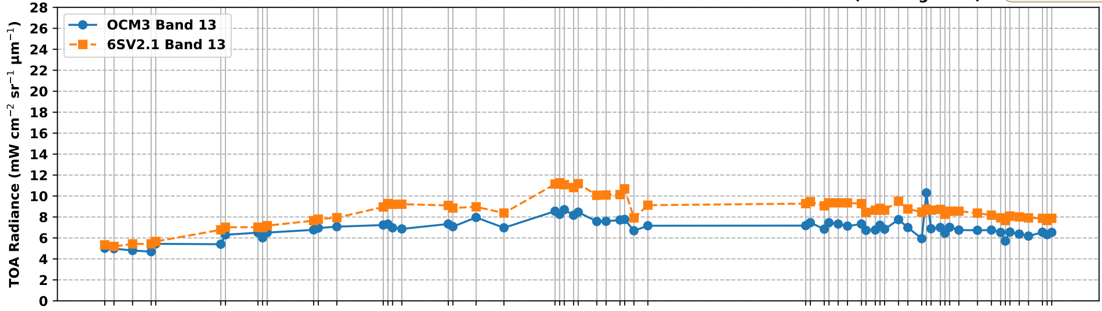
OCM3 Band 13 vs 6S Simulated Band 13 TOA Radiance over RVUS RadCalNet Site (Feb-Aug 2026)
