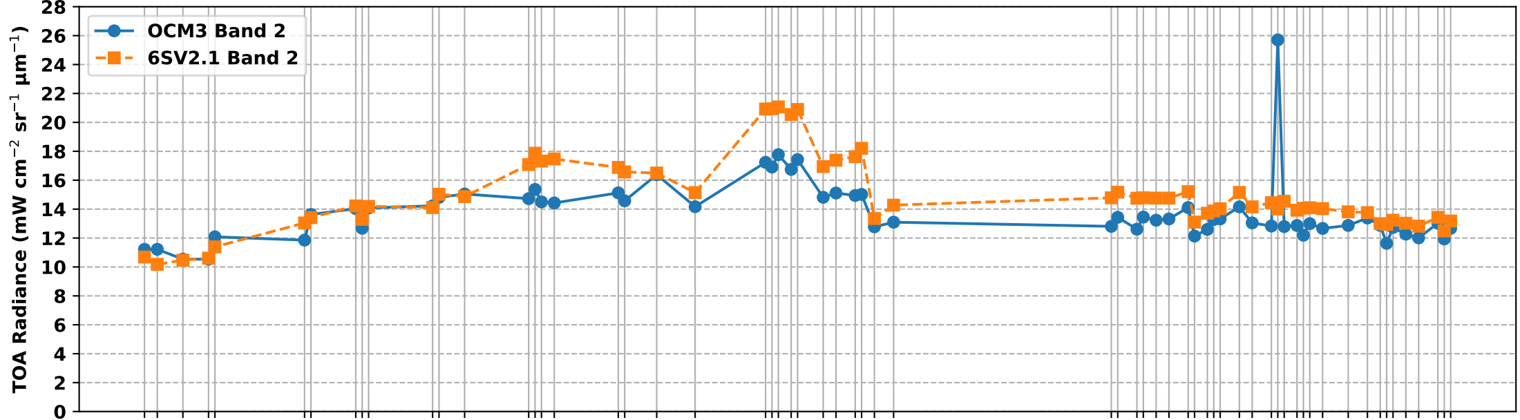
OCM3 Band 2 vs 6S Simulated Band 2 TOA Radiance over RVUS RadCalNet Site (Feb-Aug 2026)
