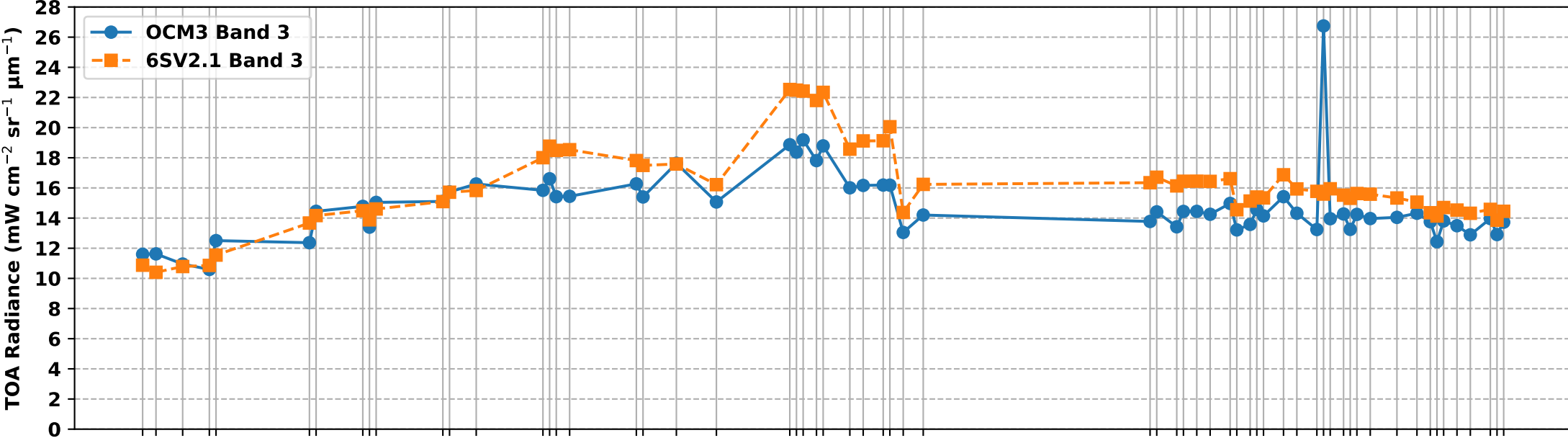
OCM3 Band 3 vs 6S Simulated Band 3 TOA Radiance over RVUS RadCalNet Site (Feb-Aug 2026)
