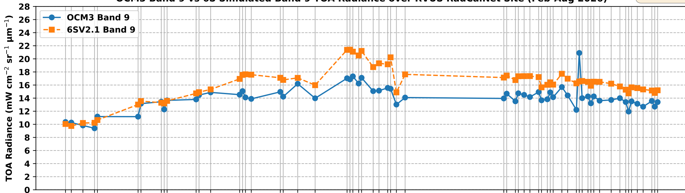
OCM3 Band 9 vs 6S Simulated Band 9 TOA Radiance over RVUS RadCalNet Site (Feb-Aug 2026)
