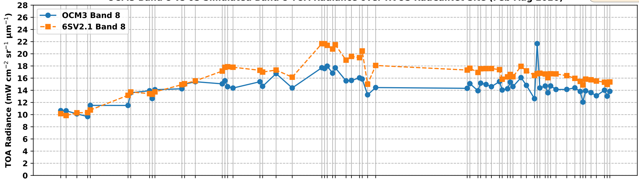
OCM3 Band 8 vs 6S Simulated Band 8 TOA Radiance over RVUS RadCalNet Site (Feb-Aug 2026)
