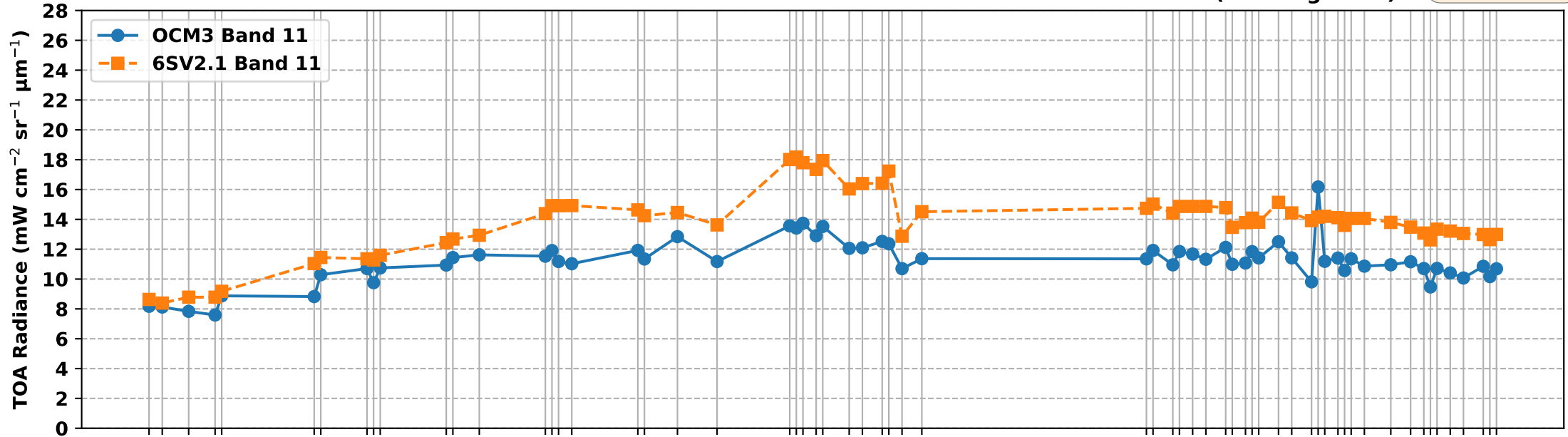
OCM3 Band 11 vs 6S Simulated Band 11 TOA Radiance over RVUS RadCalNet Site (Feb-Aug 2026)
