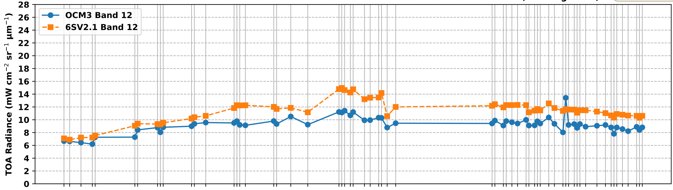
OCM3 Band 12 vs 6S Simulated Band 12 TOA Radiance over RVUS RadCalNet Site (Feb-Aug 2026)
