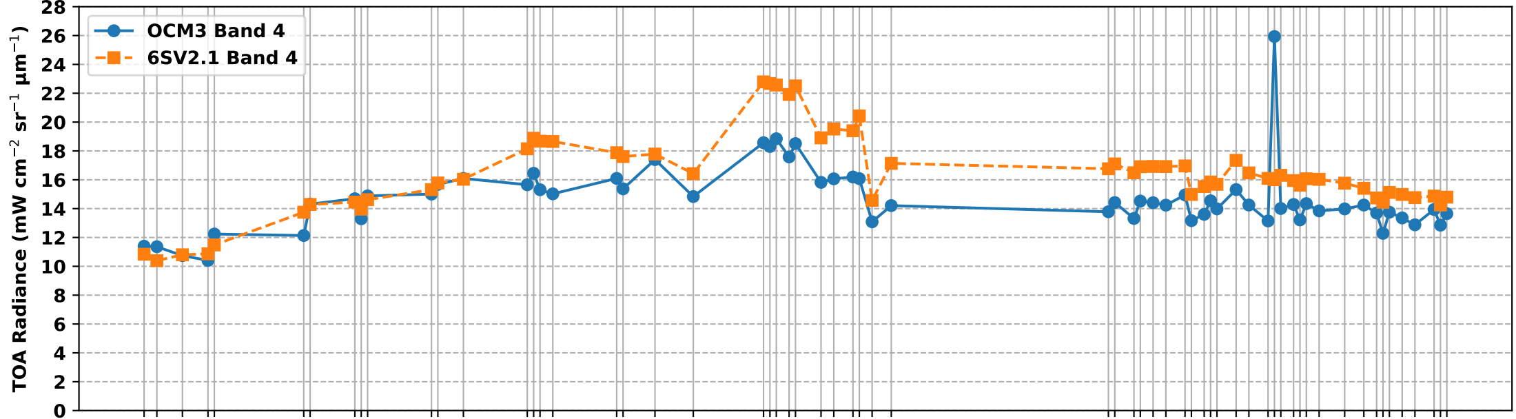
OCM3 Band 4 vs 6S Simulated Band 4 TOA Radiance over RVUS RadCalNet Site (Feb-Aug 2026)
