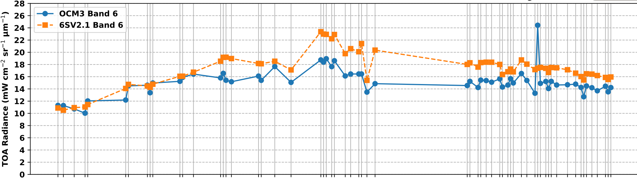
OCM3 Band 6 vs 6S Simulated Band 6 TOA Radiance over RVUS RadCalNet Site (Feb-Aug 2026)
