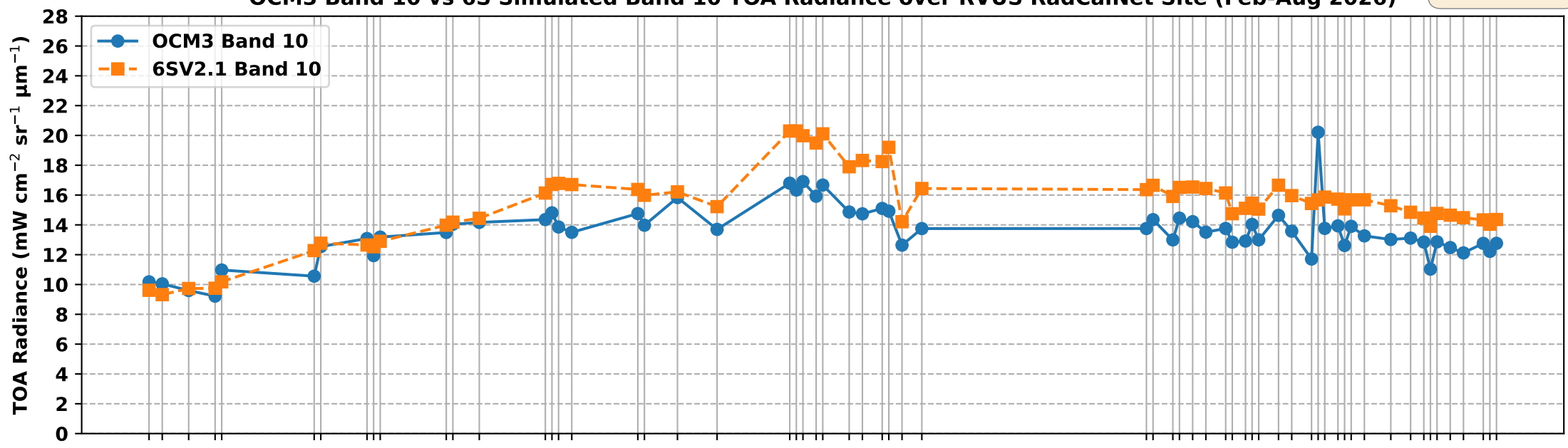
OCM3 Band 10 vs 6S Simulated Band 10 TOA Radiance over RVUS RadCalNet Site (Feb-Aug 2026)
