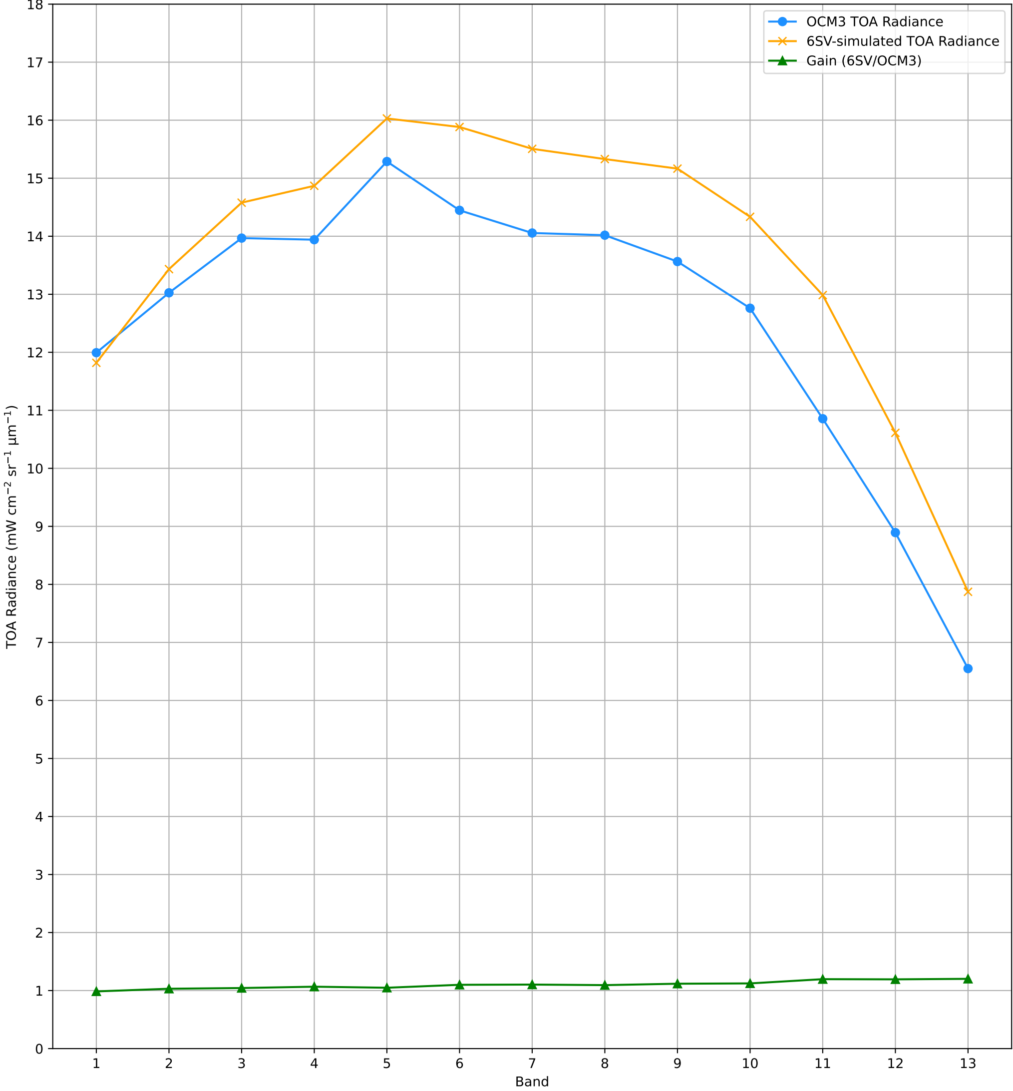
TOA Radiance (OCM3 vs. 6SV) over RVUS RadCalNet Site Lat: 38.497°, Lon: -115.69° - 23-AUG-2026 (STRIP_ID: 19763)
