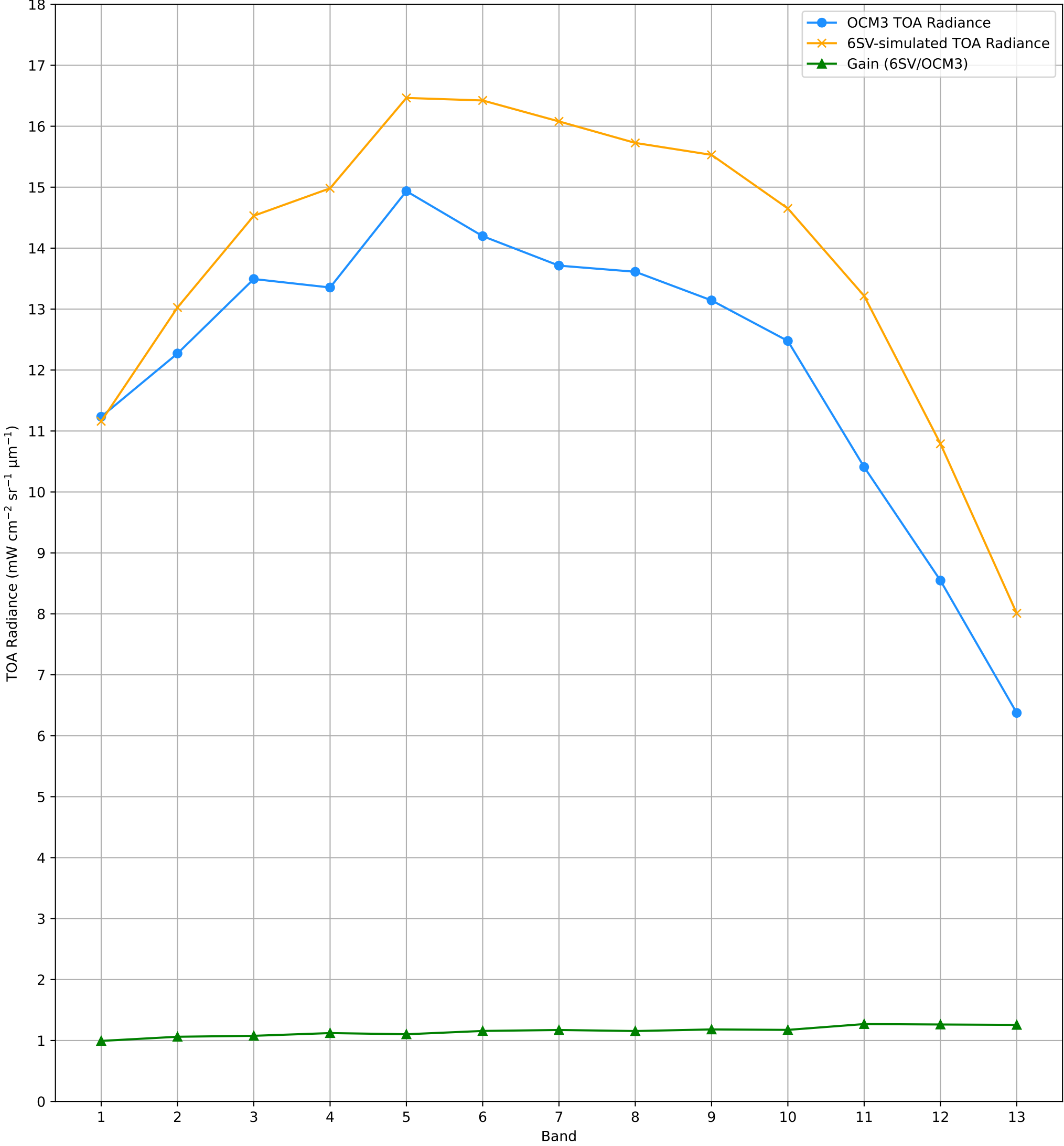
TOA Radiance (OCM3 vs. 6SV) over RVUS RadCalNet Site Lat: 38.497°, Lon: -115.69° - 18-AUG-2026 (STRIP_ID: 19691)
