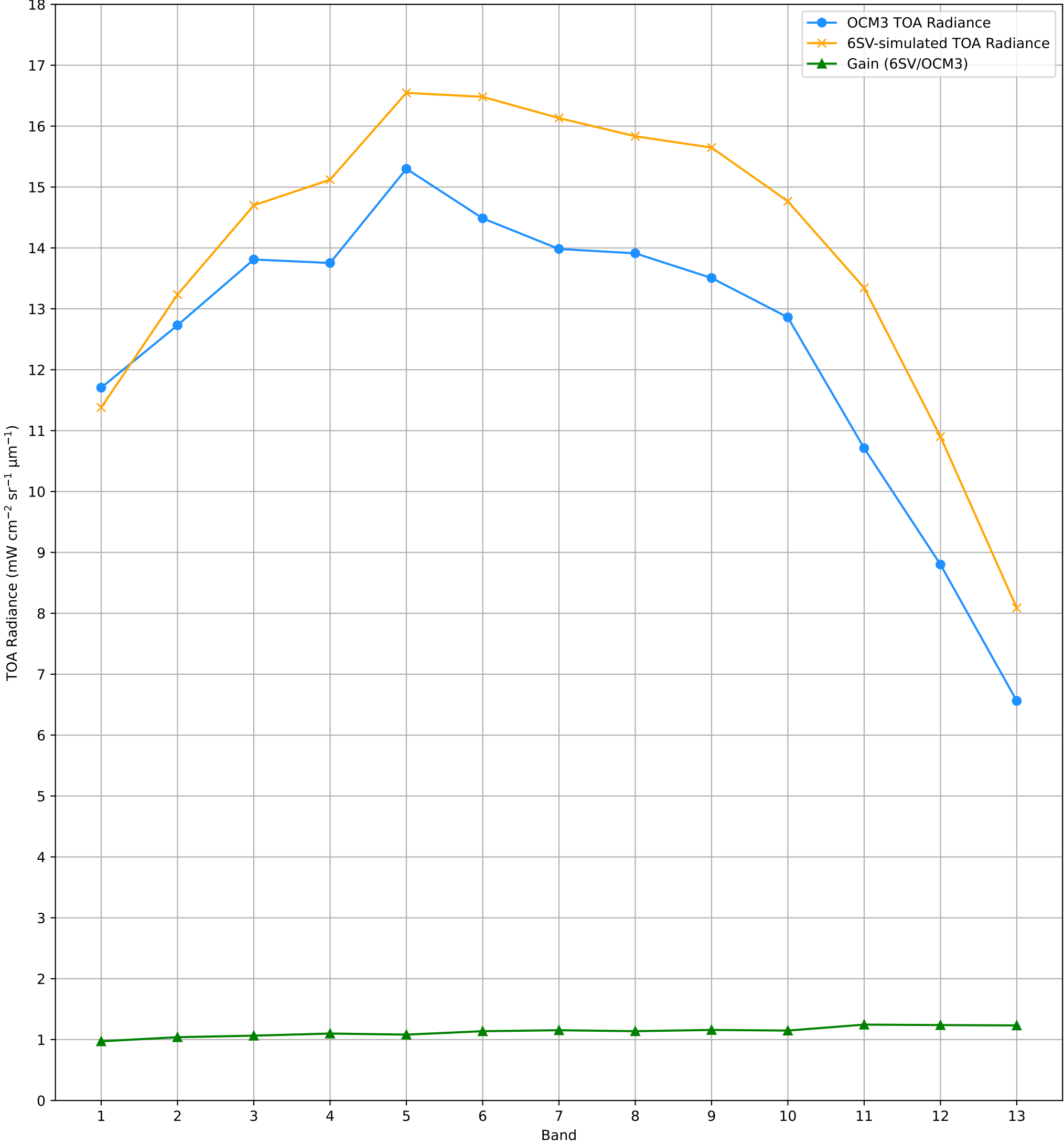
TOA Radiance (OCM3 vs. 6SV) over RVUS RadCalNet Site Lat: 38.497°, Lon: -115.69° - 16-AUG-2026 (STRIP_ID: 19662)
