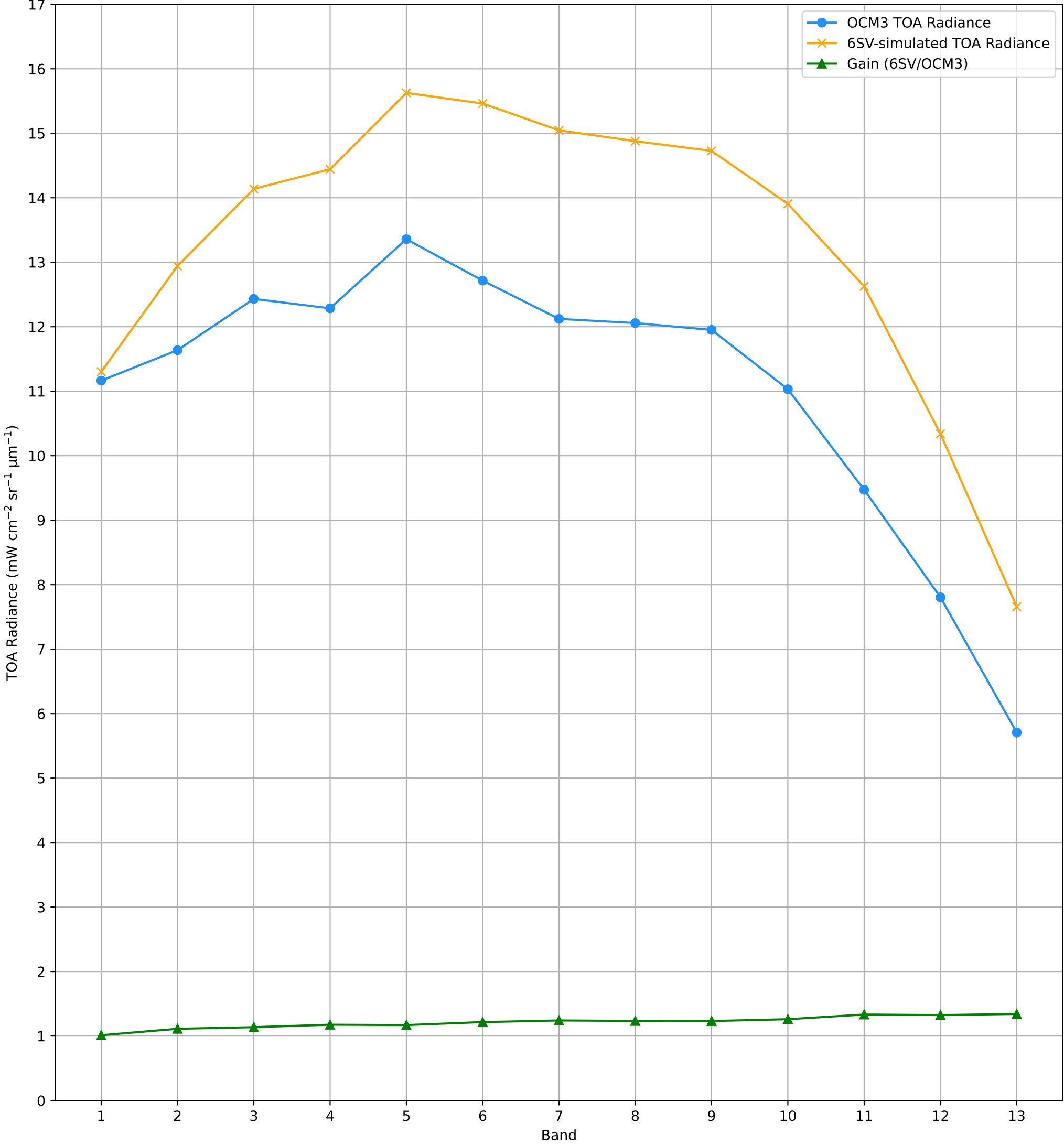
TOA Radiance (OCM3 vs. 6SV) over RVUS RadCalNet Site Lat: 38.497°, Lon: -115.69° - 15-AUG-2026 (STRIP_ID: 19648)
