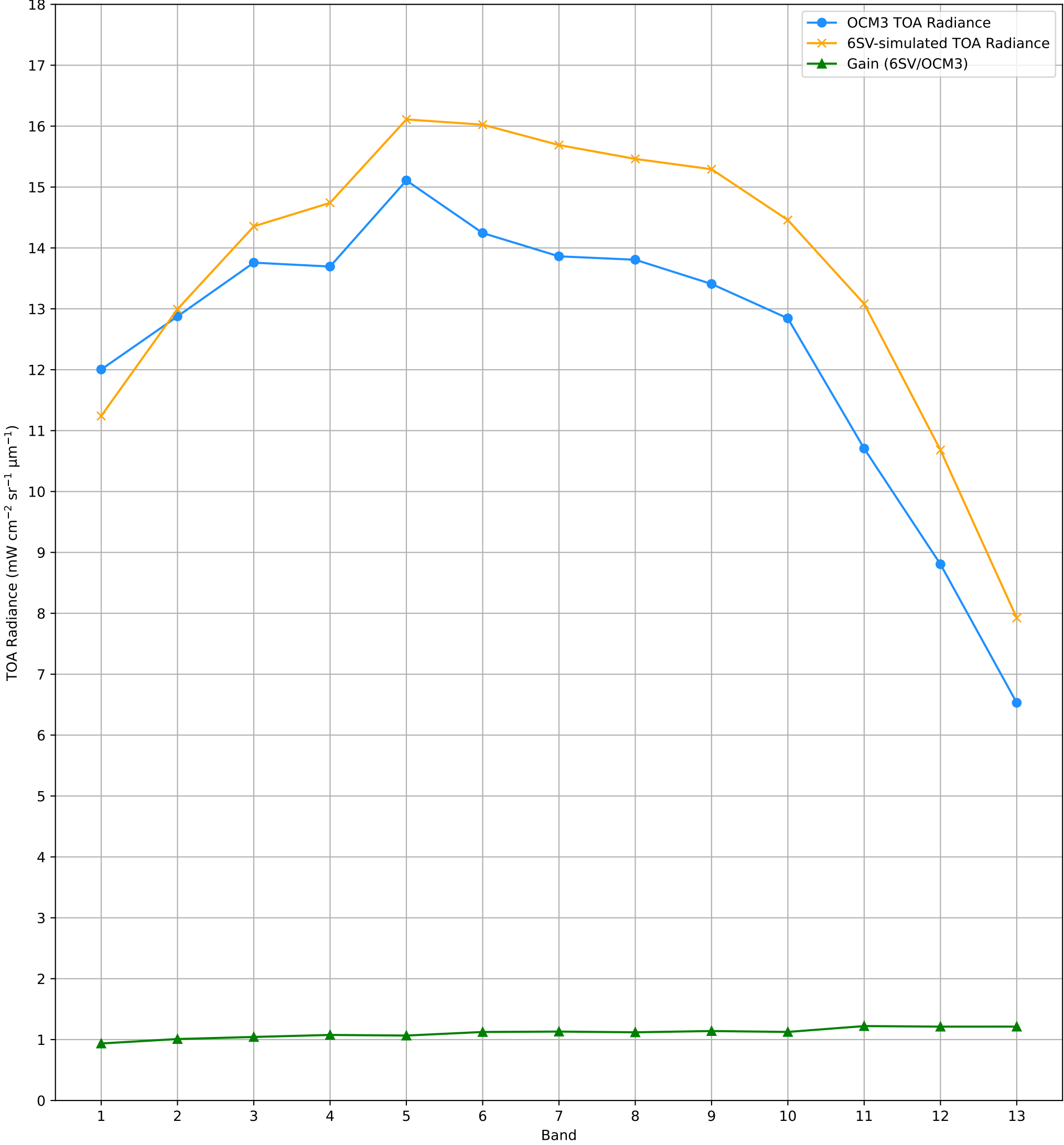
TOA Radiance (OCM3 vs. 6SV) over RVUS RadCalNet Site Lat: 38.497°, Lon: -115.69° - 14-AUG-2026 (STRIP_ID: 19633)
