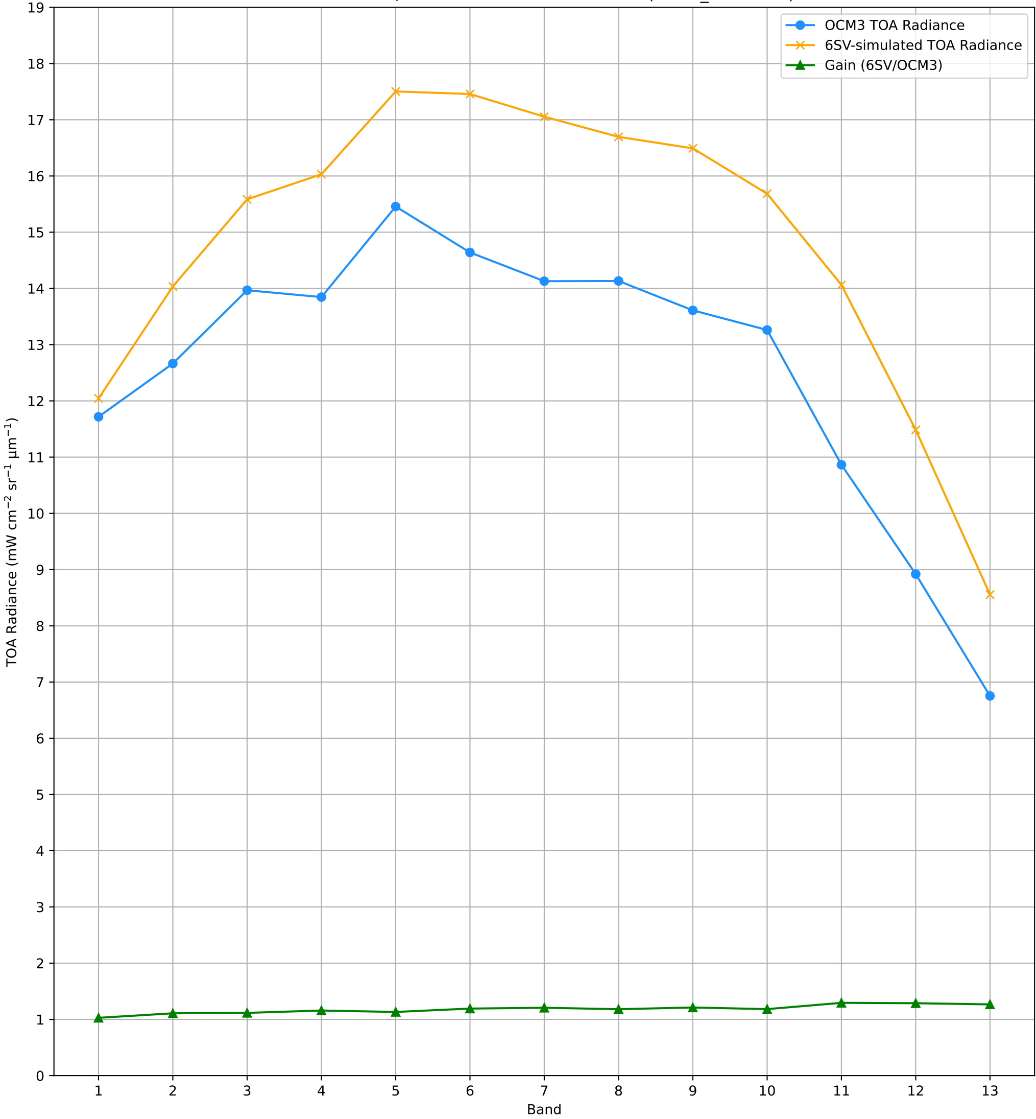
TOA Radiance (OCM3 vs. 6SV) over RVUS RadCalNet Site Lat: 38.497°, Lon: -115.69° - 05-AUG-2026 (STRIP_ID: 19503)
