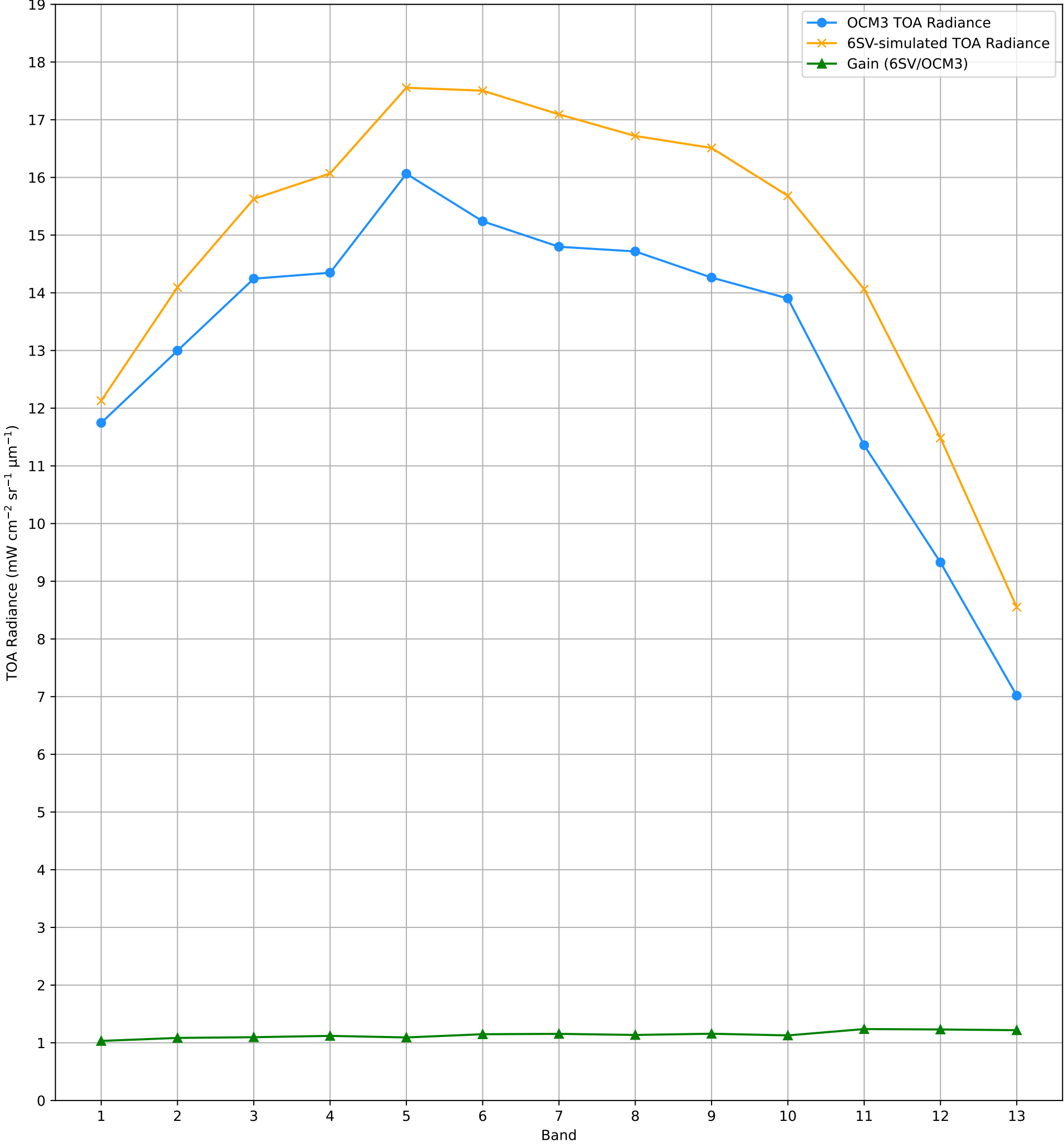
TOA Radiance (OCM3 vs. 6SV) over RVUS RadCalNet Site Lat: 38.497°, Lon: -115.69° - 03-AUG-2026 (STRIP_ID: 19474)
