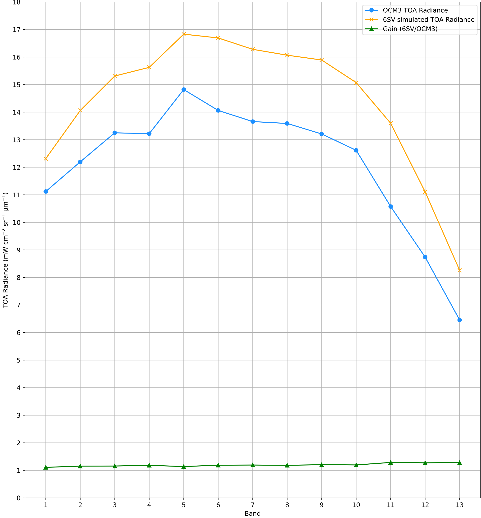
TOA Radiance (OCM3 vs. 6SV) over RVUS RadCalNet Site Lat: 38.497°, Lon: -115.69° - 02-AUG-2026 (STRIP_ID: 19460)
