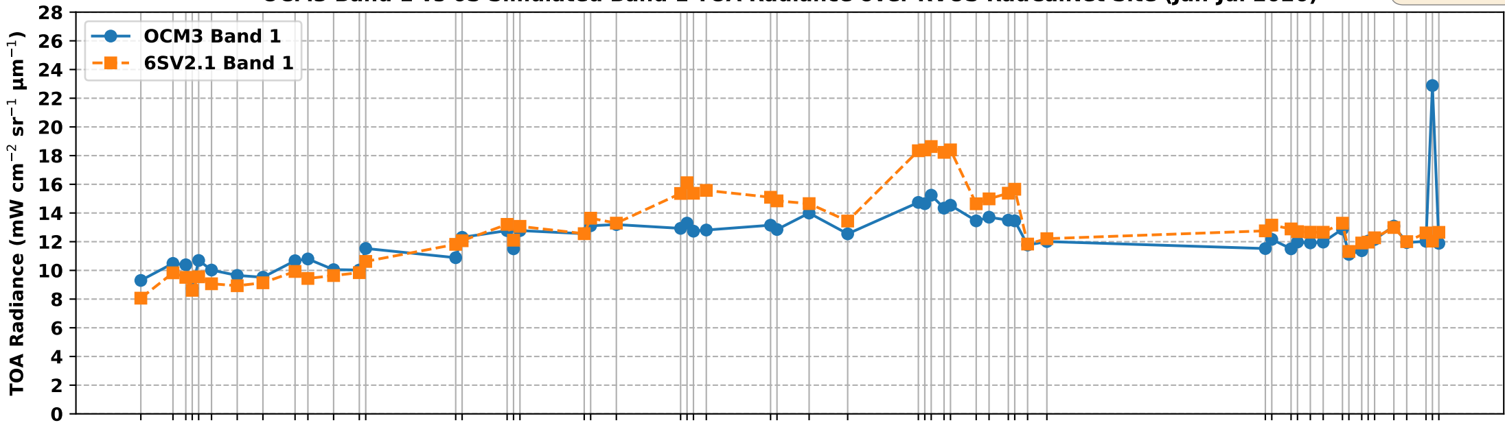
OCM3 Band 1 vs 6S Simulated Band 1 TOA Radiance over RVUS RadCalNet Site (Jan-Jul 2026)
