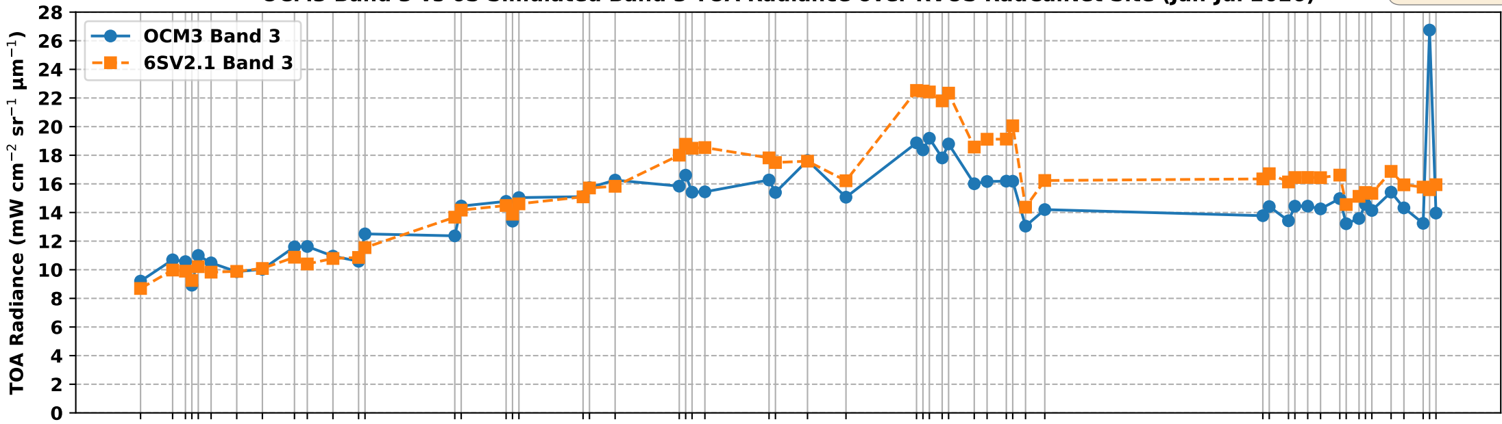
OCM3 Band 3 vs 6S Simulated Band 3 TOA Radiance over RVUS RadCalNet Site (Jan-Jul 2026)
