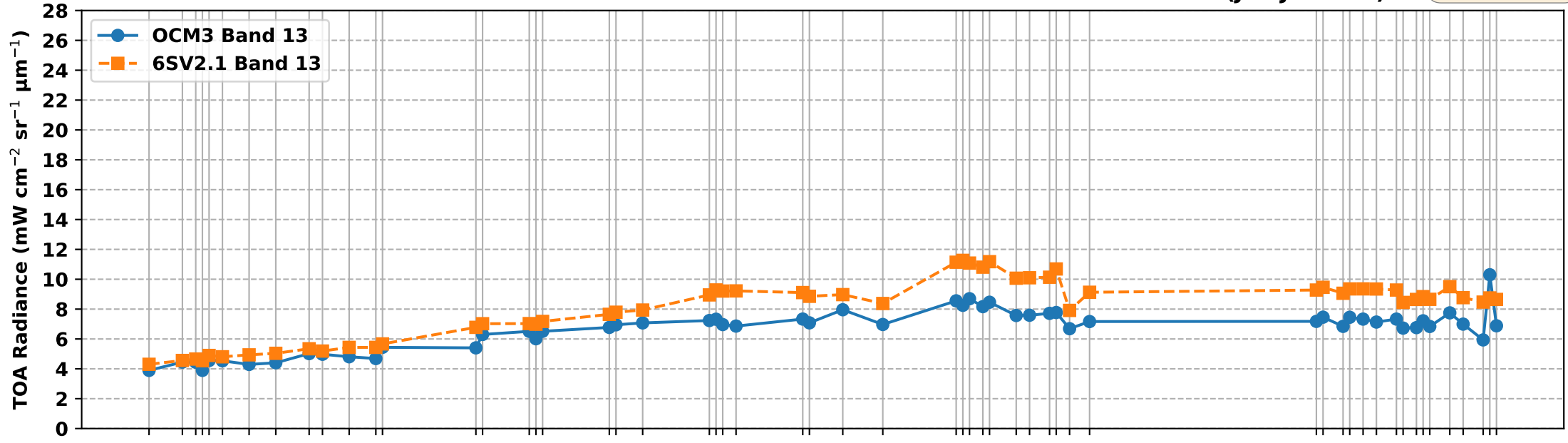
OCM3 Band 13 vs 6S Simulated Band 13 TOA Radiance over RVUS RadCalNet Site (Jan-Jul 2026)
