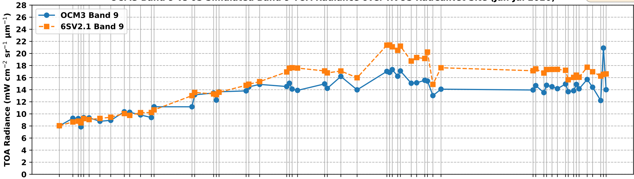
OCM3 Band 9 vs 6S Simulated Band 9 TOA Radiance over RVUS RadCalNet Site (Jan-Jul 2026)
