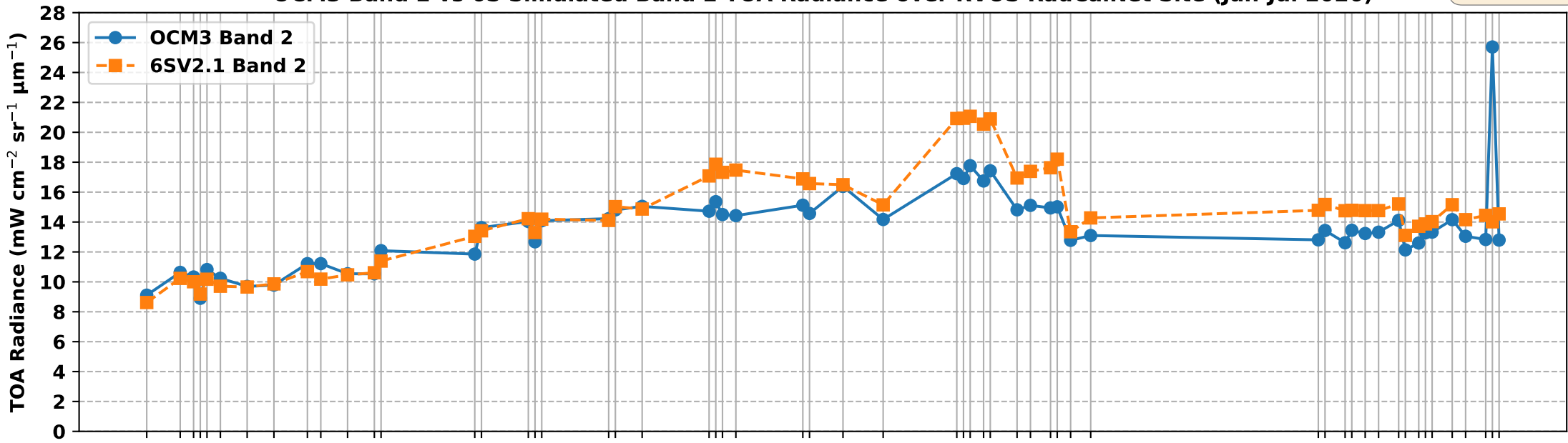
OCM3 Band 2 vs 6S Simulated Band 2 TOA Radiance over RVUS RadCalNet Site (Jan-Jul 2026)
