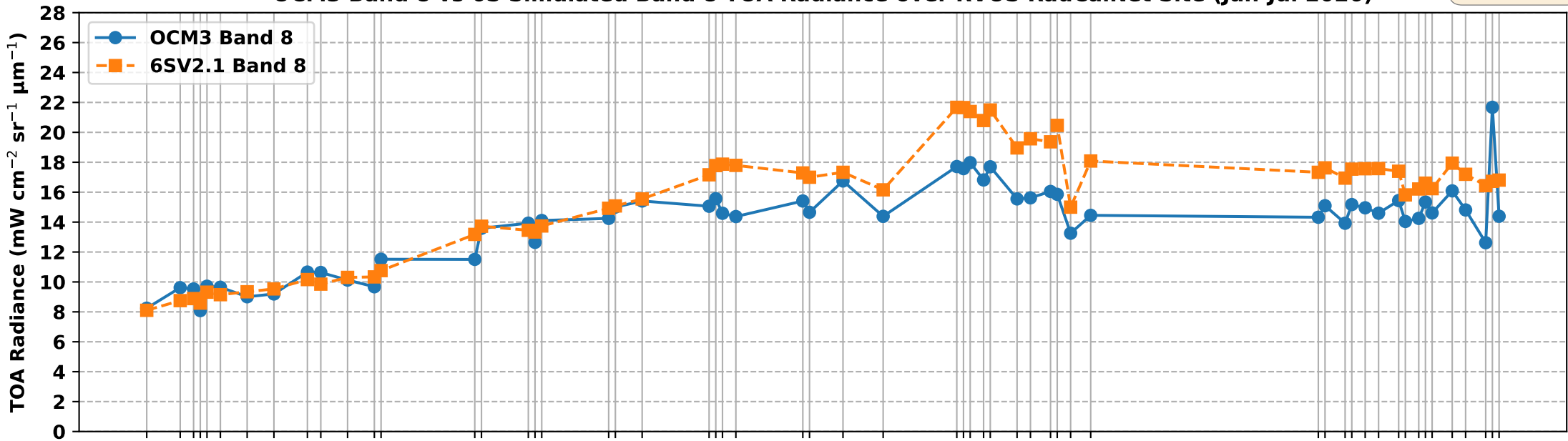
OCM3 Band 8 vs 6S Simulated Band 8 TOA Radiance over RVUS RadCalNet Site (Jan-Jul 2026)
