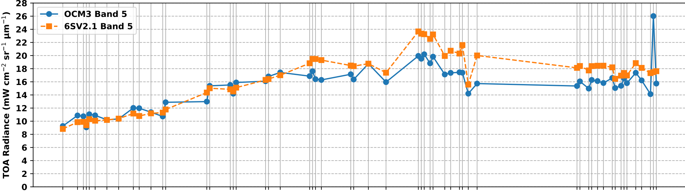
OCM3 Band 5 vs 6S Simulated Band 5 TOA Radiance over RVUS RadCalNet Site (Jan-Jul 2026)
