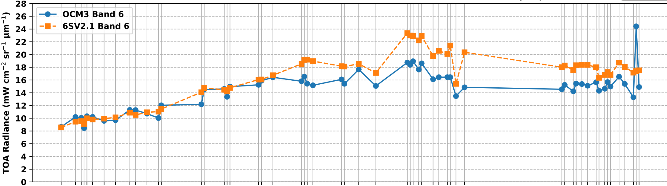
OCM3 Band 6 vs 6S Simulated Band 6 TOA Radiance over RVUS RadCalNet Site (Jan-Jul 2026)
