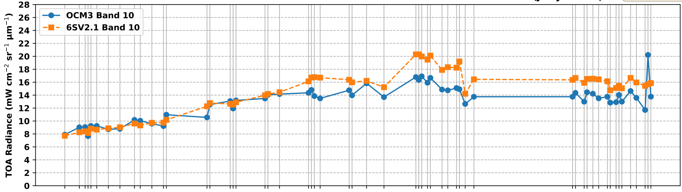
OCM3 Band 10 vs 6S Simulated Band 10 TOA Radiance over RVUS RadCalNet Site (Jan-Jul 2026)
