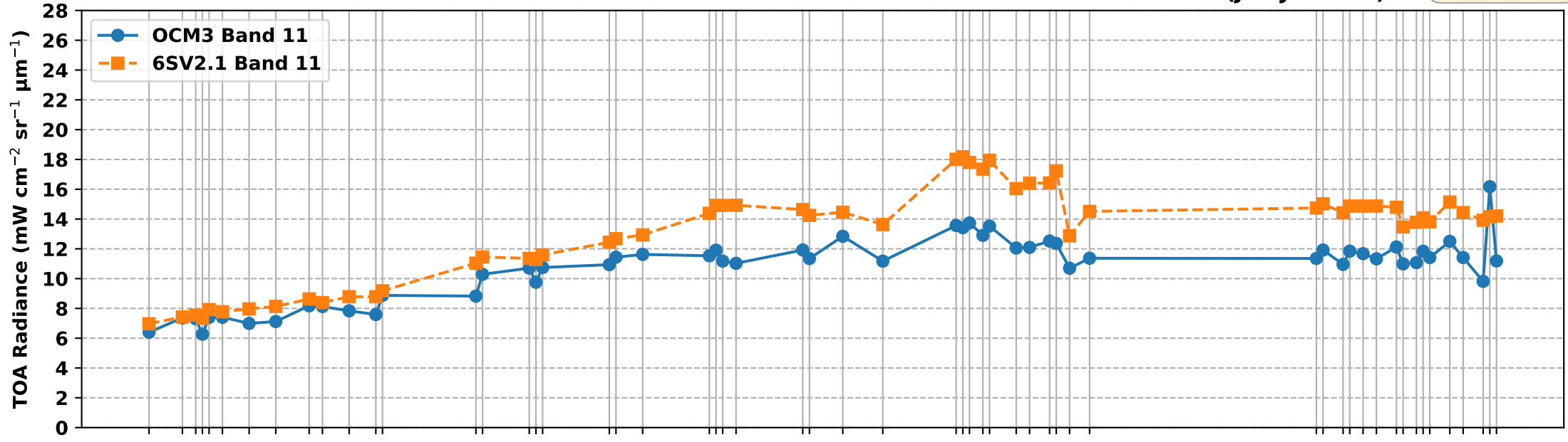
OCM3 Band 11 vs 6S Simulated Band 11 TOA Radiance over RVUS RadCalNet Site (Jan-Jul 2026)
