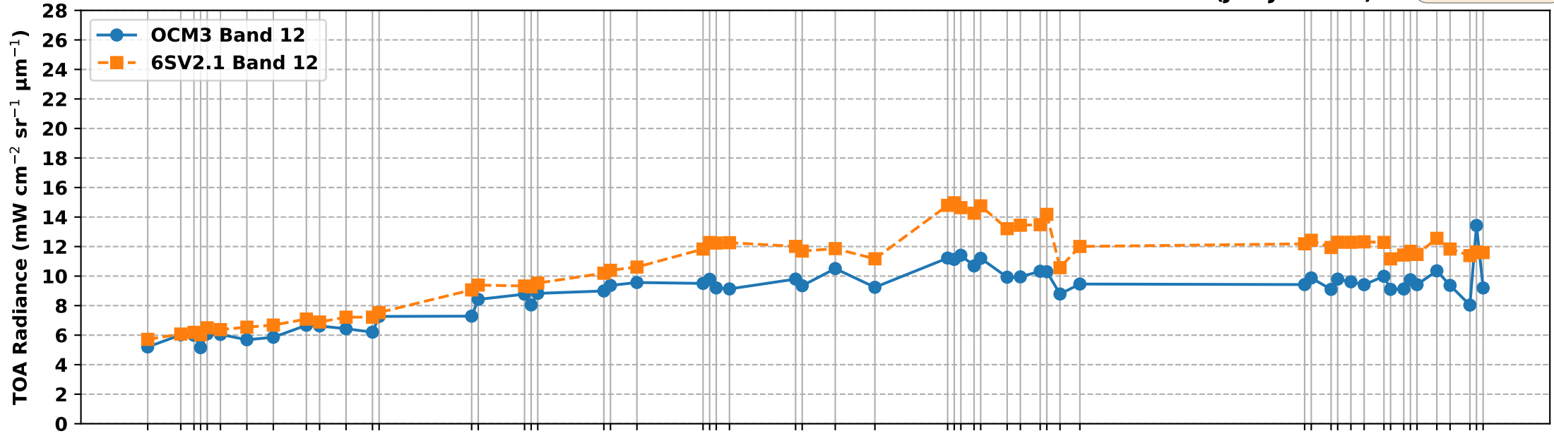
OCM3 Band 12 vs 6S Simulated Band 12 TOA Radiance over RVUS RadCalNet Site (Jan-Jul 2026)
