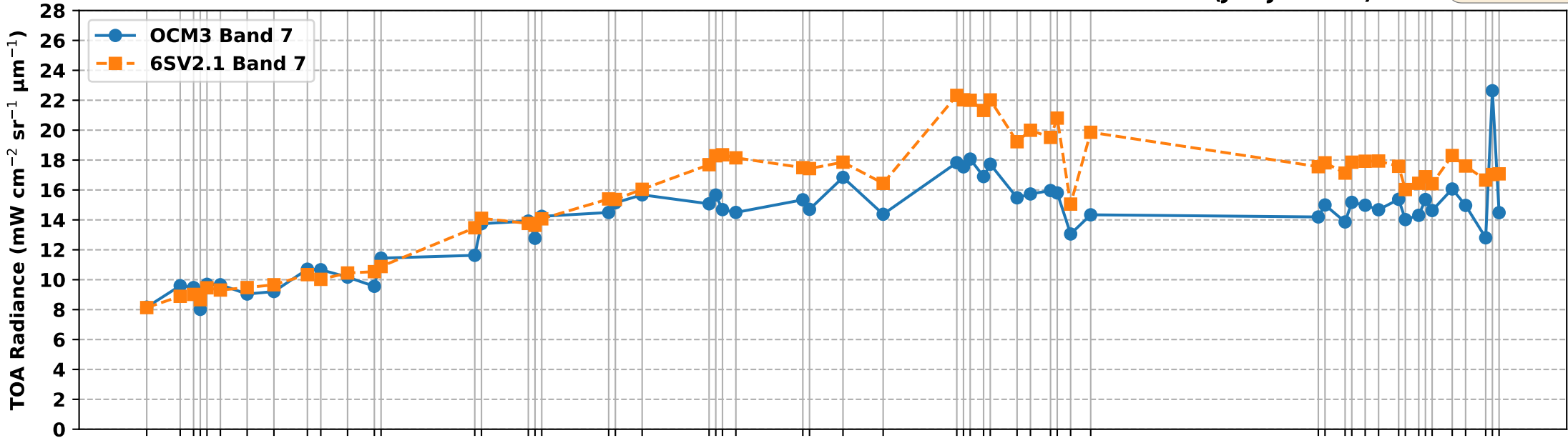
OCM3 Band 7 vs 6S Simulated Band 7 TOA Radiance over RVUS RadCalNet Site (Jan-Jul 2026)
