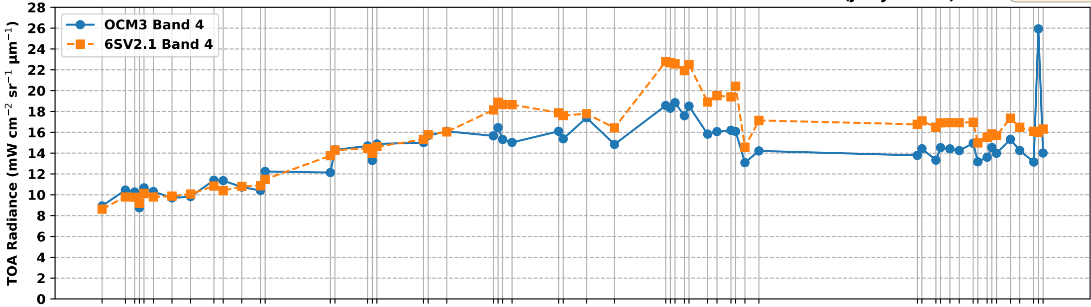
OCM3 Band 4 vs 6S Simulated Band 4 TOA Radiance over RVUS RadCalNet Site (Jan-Jul 2026)
