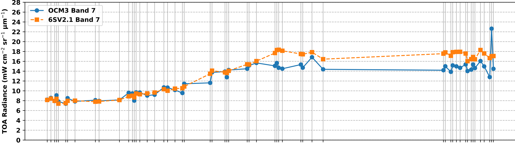
OCM3 Band 7 vs 6S Simulated Band 7 TOA Radiance over RVUS RadCalNet Site (Dec 2025 to Jul 2026)
