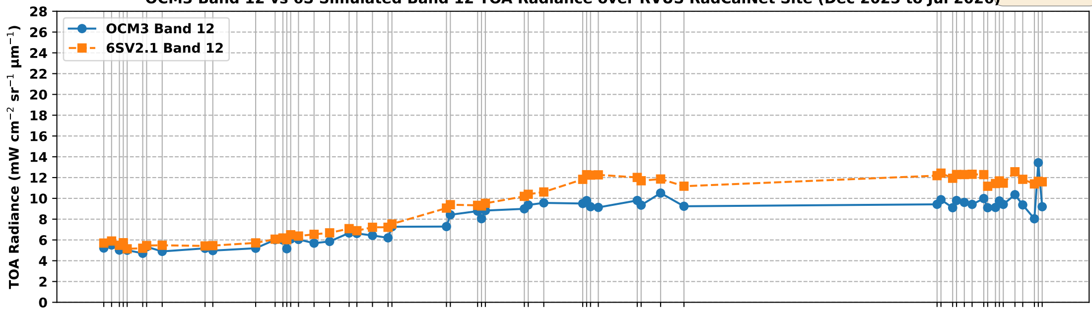
OCM3 Band 12 vs 6S Simulated Band 12 TOA Radiance over RVUS RadCalNet Site (Dec 2025 to Jul 2026)
