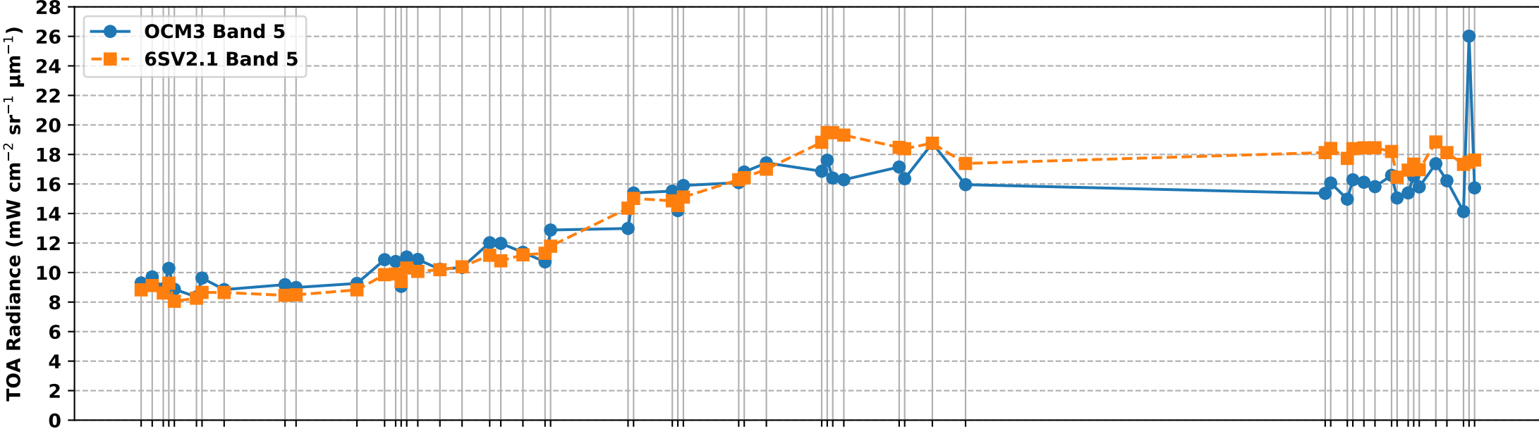
OCM3 Band 5 vs 6S Simulated Band 5 TOA Radiance over RVUS RadCalNet Site (Dec 2025 to Jul 2026)
