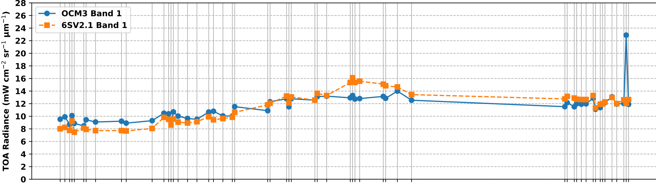
OCM3 Band 1 vs 6S Simulated Band 1 TOA Radiance over RVUS RadCalNet Site (Dec 2025 to Jul 2026)
