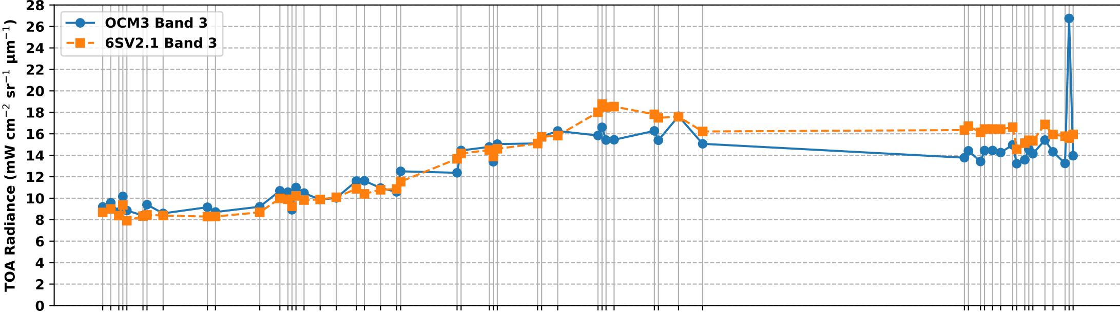
OCM3 Band 3 vs 6S Simulated Band 3 TOA Radiance over RVUS RadCalNet Site (Dec 2025 to Jul 2026)
