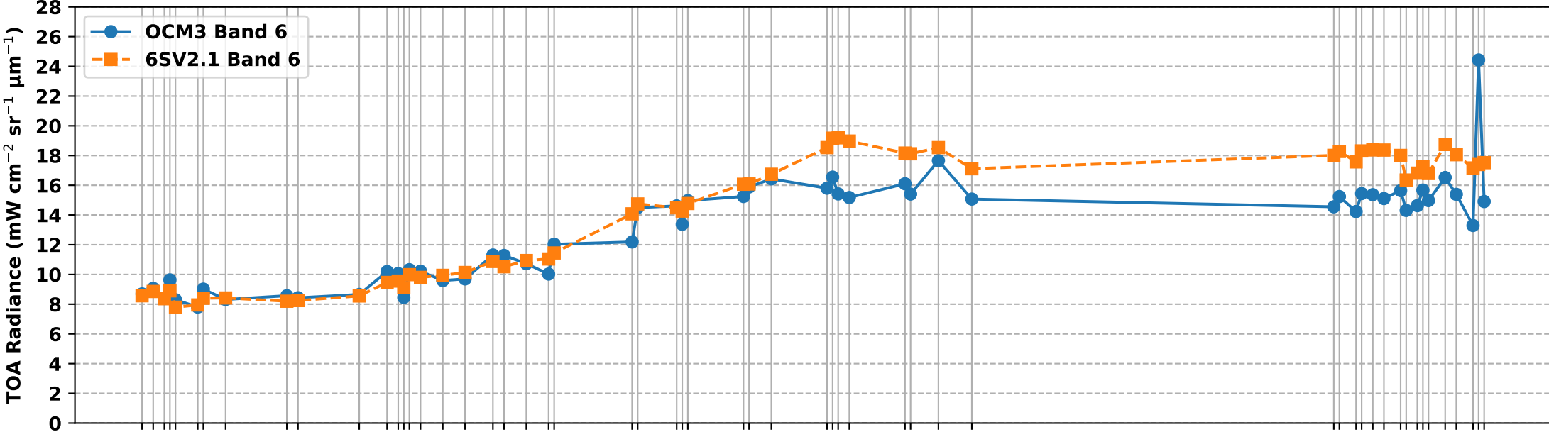
OCM3 Band 6 vs 6S Simulated Band 6 TOA Radiance over RVUS RadCalNet Site (Dec 2025 to Jul 2026)
