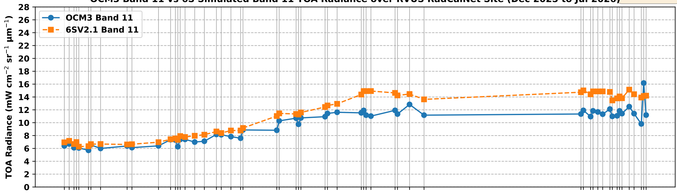
OCM3 Band 11 vs 6S Simulated Band 11 TOA Radiance over RVUS RadCalNet Site (Dec 2025 to Jul 2026)
