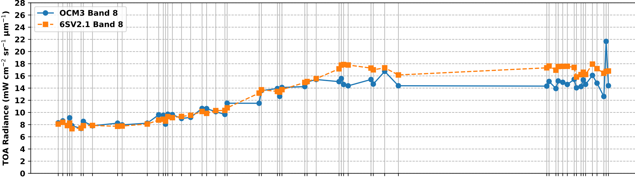
OCM3 Band 8 vs 6S Simulated Band 8 TOA Radiance over RVUS RadCalNet Site (Dec 2025 to Jul 2026)
