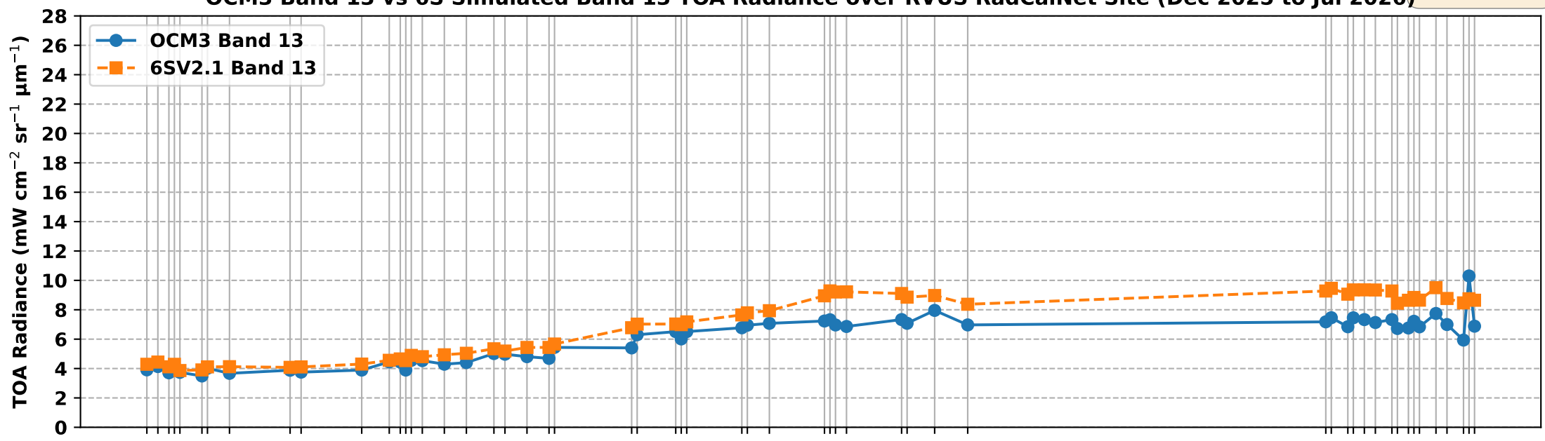
OCM3 Band 13 vs 6S Simulated Band 13 TOA Radiance over RVUS RadCalNet Site (Dec 2025 to Jul 2026)
