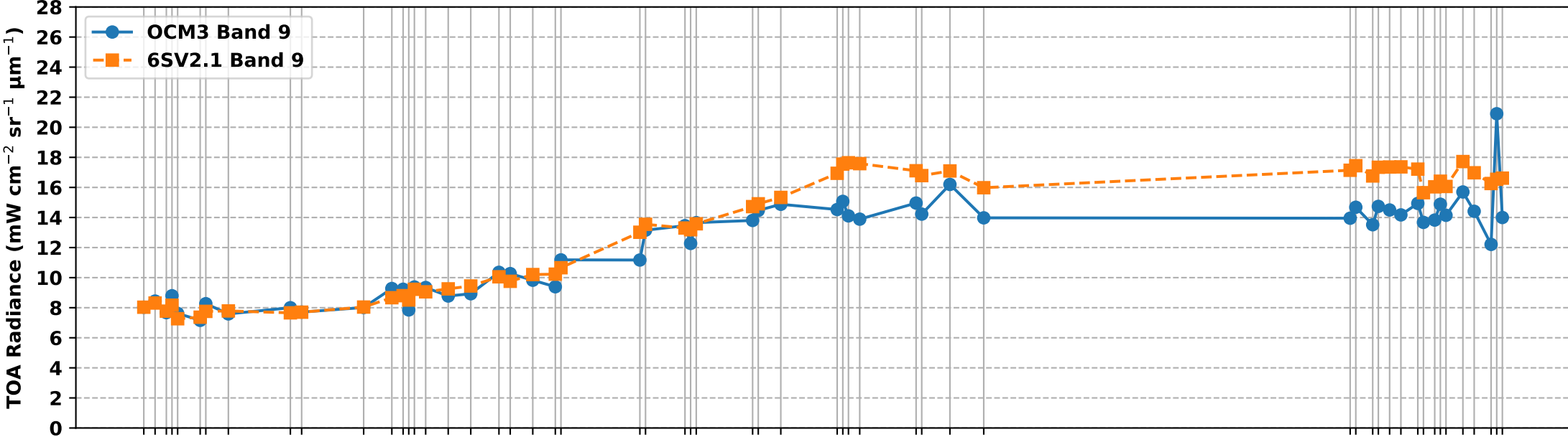
OCM3 Band 9 vs 6S Simulated Band 9 TOA Radiance over RVUS RadCalNet Site (Dec 2025 to Jul 2026)
