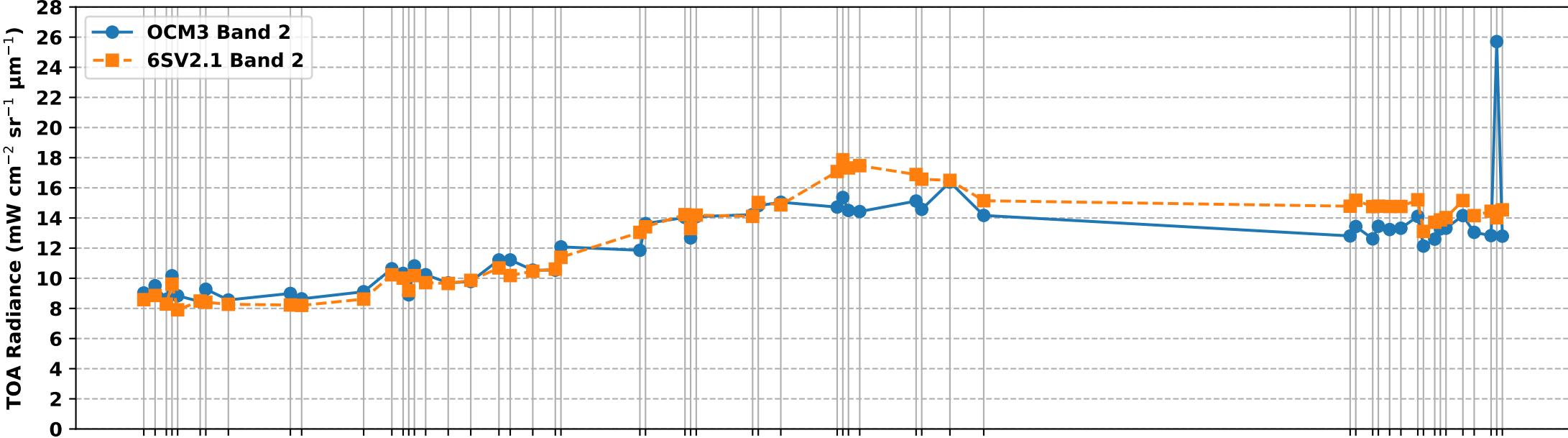
OCM3 Band 2 vs 6S Simulated Band 2 TOA Radiance over RVUS RadCalNet Site (Dec 2025 to Jul 2026)
