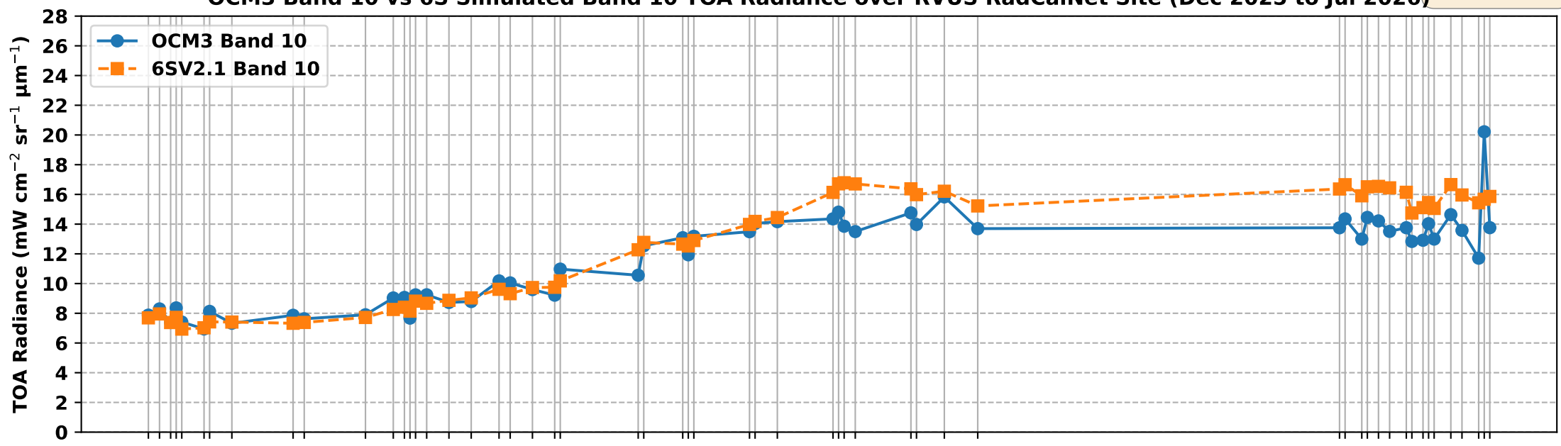
OCM3 Band 10 vs 6S Simulated Band 10 TOA Radiance over RVUS RadCalNet Site (Dec 2025 to Jul 2026)
