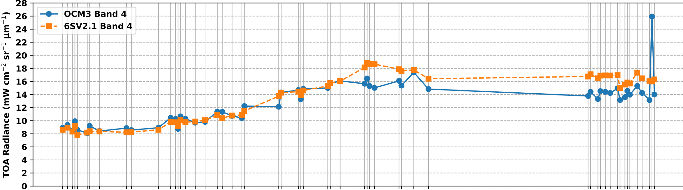
OCM3 Band 4 vs 6S Simulated Band 4 TOA Radiance over RVUS RadCalNet Site (Dec 2025 to Jul 2026)
