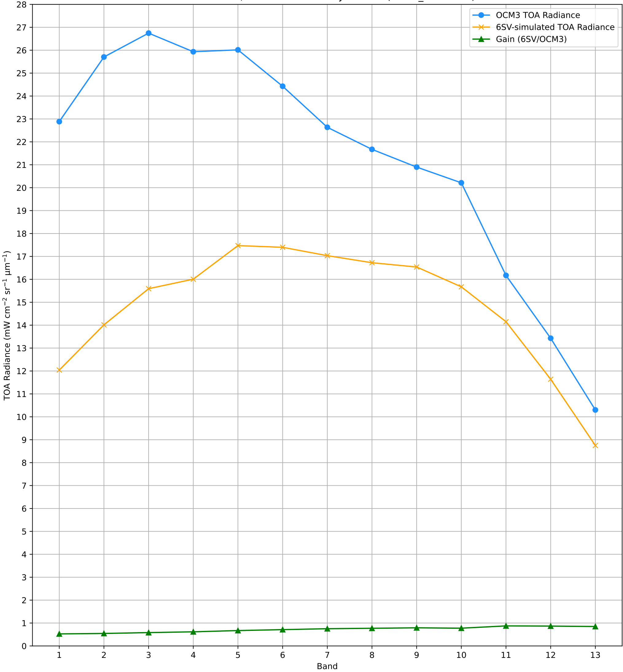
TOA Radiance (OCM3 vs. 6SV) over RVUS RadCalNet Site Lat: 38.497°, Lon: -115.69° - 29-JUL-2026 (STRIP_ID: 19402)
