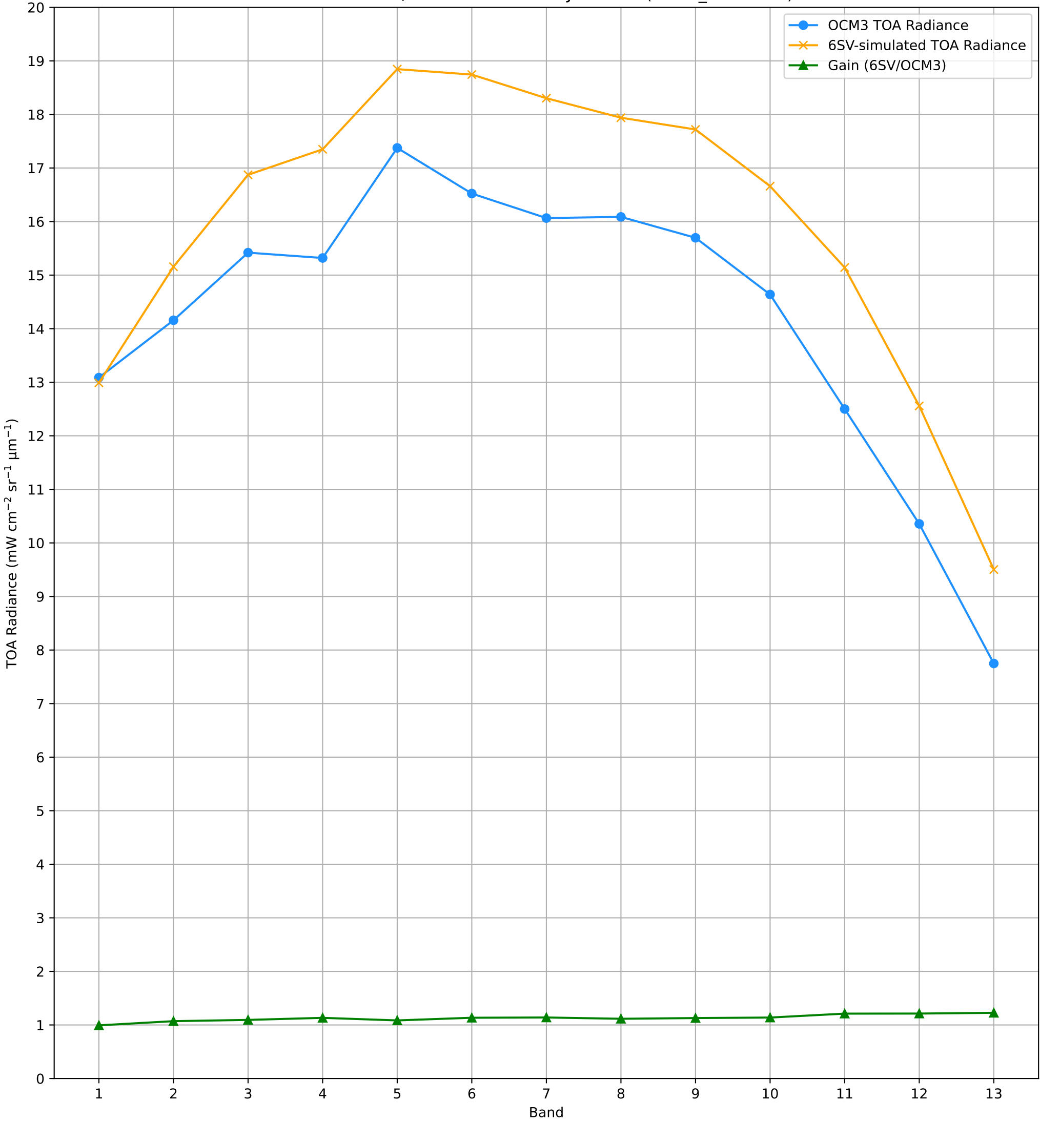
TOA Radiance (OCM3 vs. 6SV) over RVUS RadCalNet Site Lat: 38.497°, Lon: -115.69° - 23-JUL-2026 (STRIP_ID: 19315)
