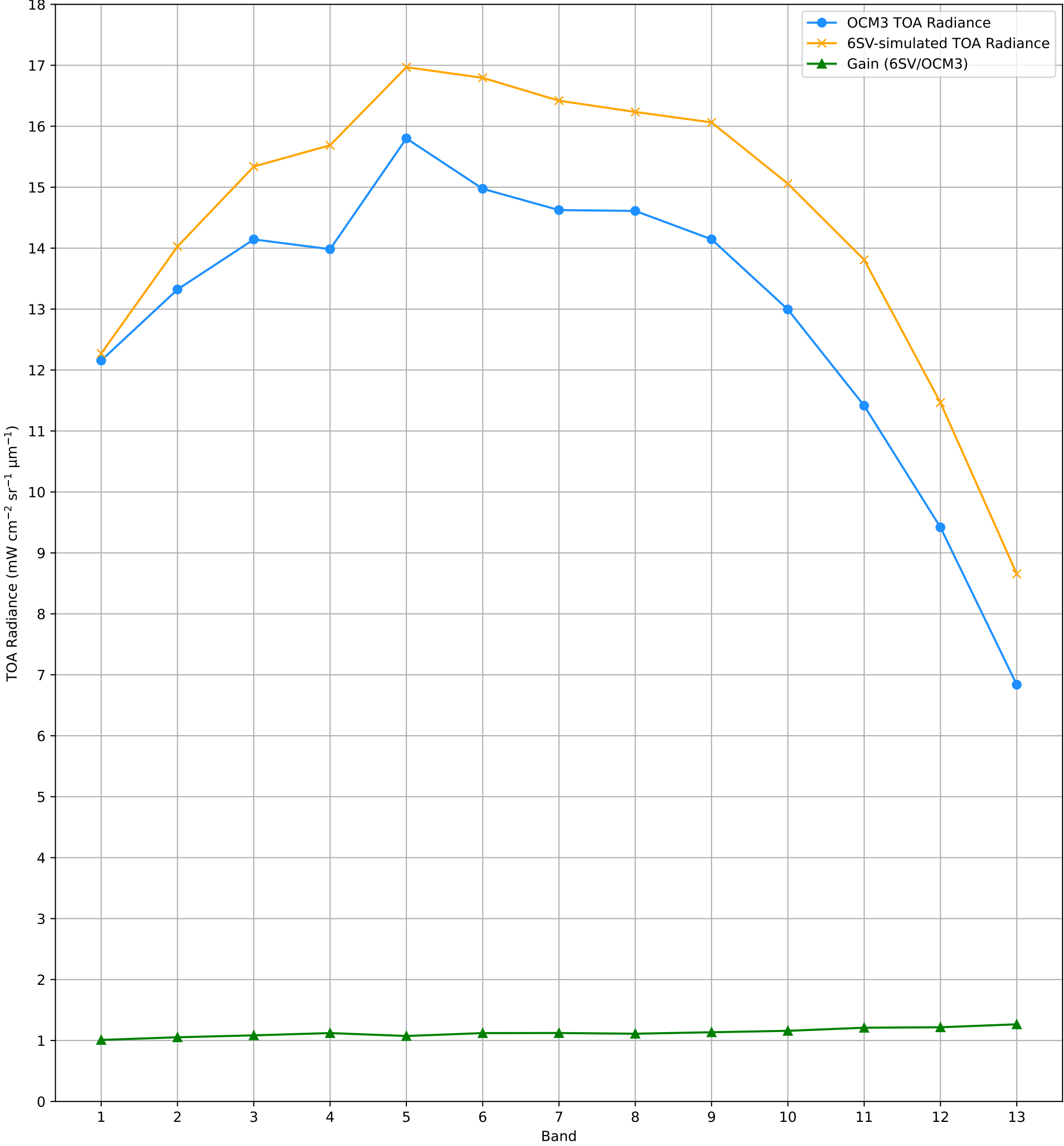
TOA Radiance (OCM3 vs. 6SV) over RVUS RadCalNet Site Lat: 38.497°, Lon: -115.69° - 20-JUL-2026 (STRIP_ID: 19272)
