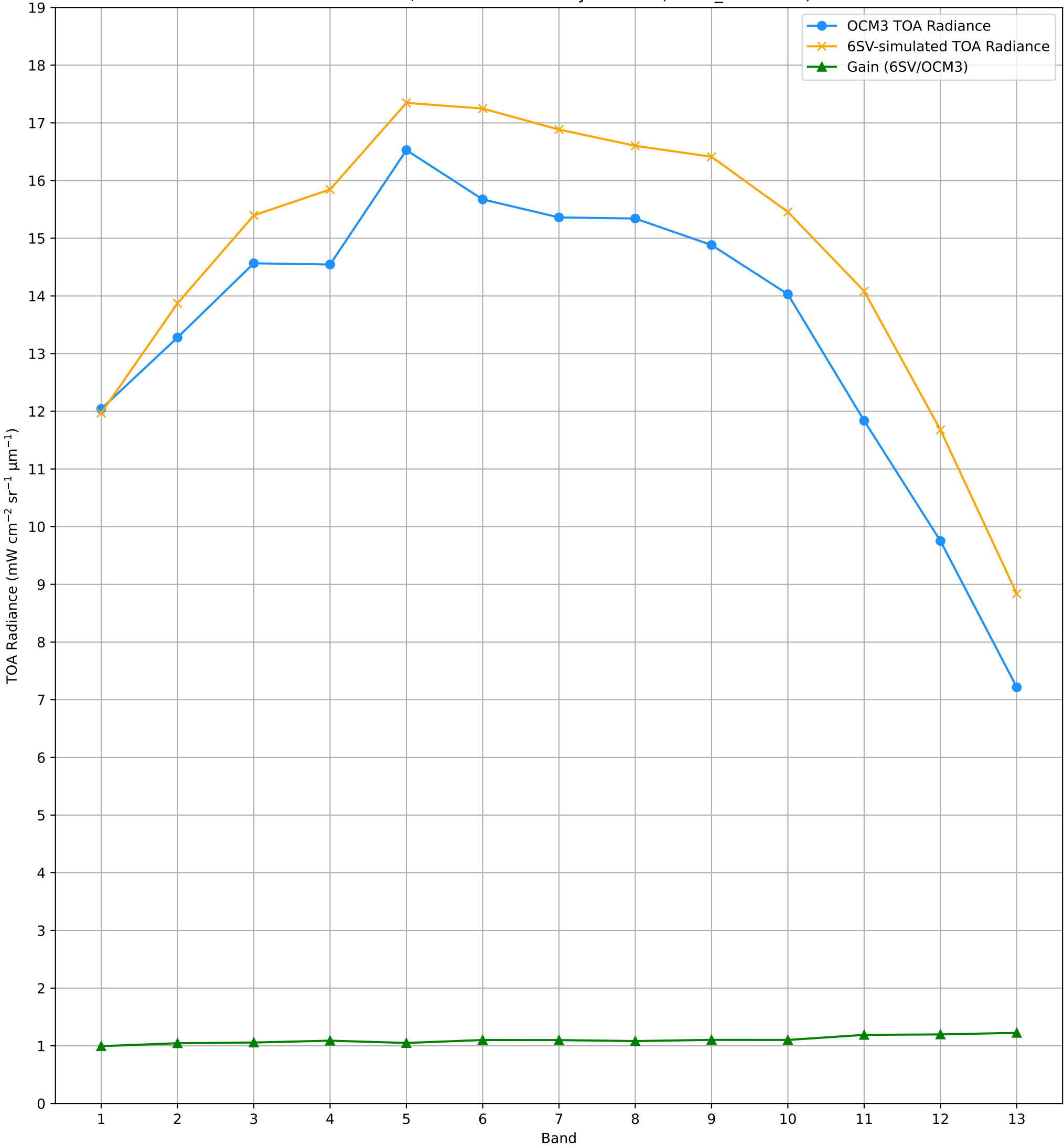
TOA Radiance (OCM3 vs. 6SV) over RVUS RadCalNet Site Lat: 38.497°, Lon: -115.69° - 19-JUL-2026 (STRIP_ID: 19257)
