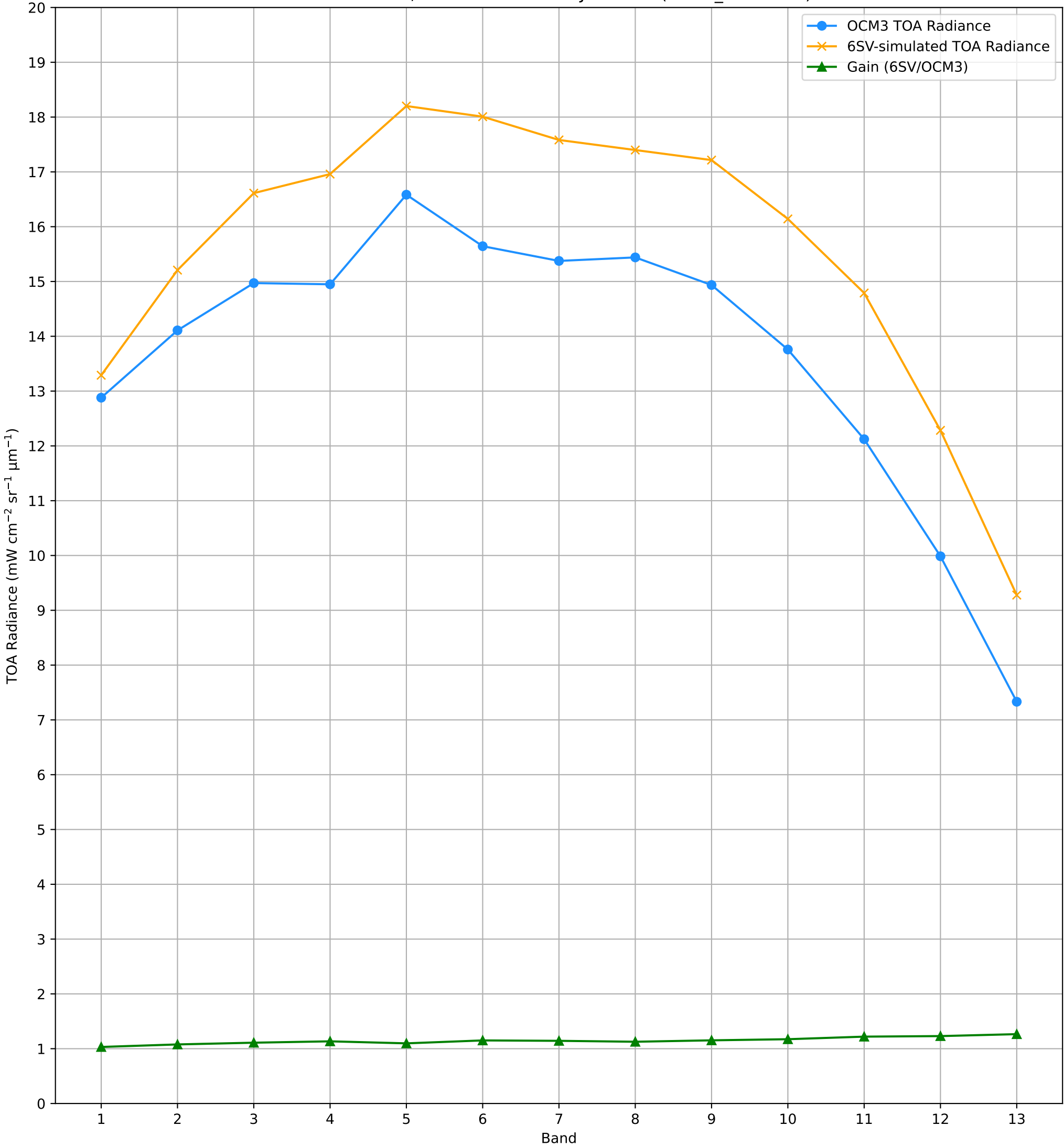
TOA Radiance (OCM3 vs. 6SV) over RVUS RadCalNet Site Lat: 38.497°, Lon: -115.69° - 15-JUL-2026 (STRIP_ID: 19199)
