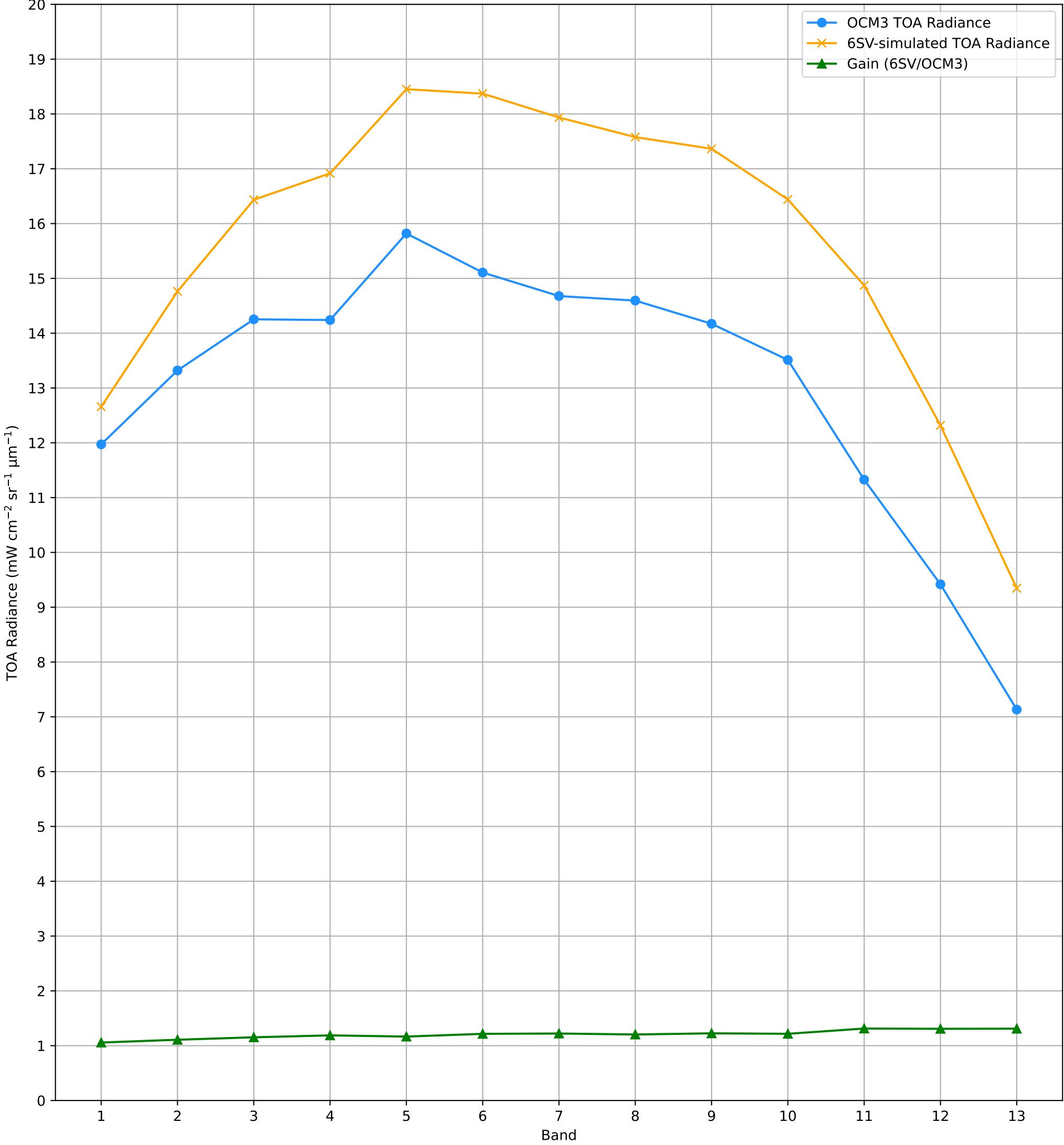
TOA Radiance (OCM3 vs. 6SV) over RVUS RadCalNet Site Lat: 38.497°, Lon: -115.69° - 12-JUL-2026 (STRIP_ID: 19156)
