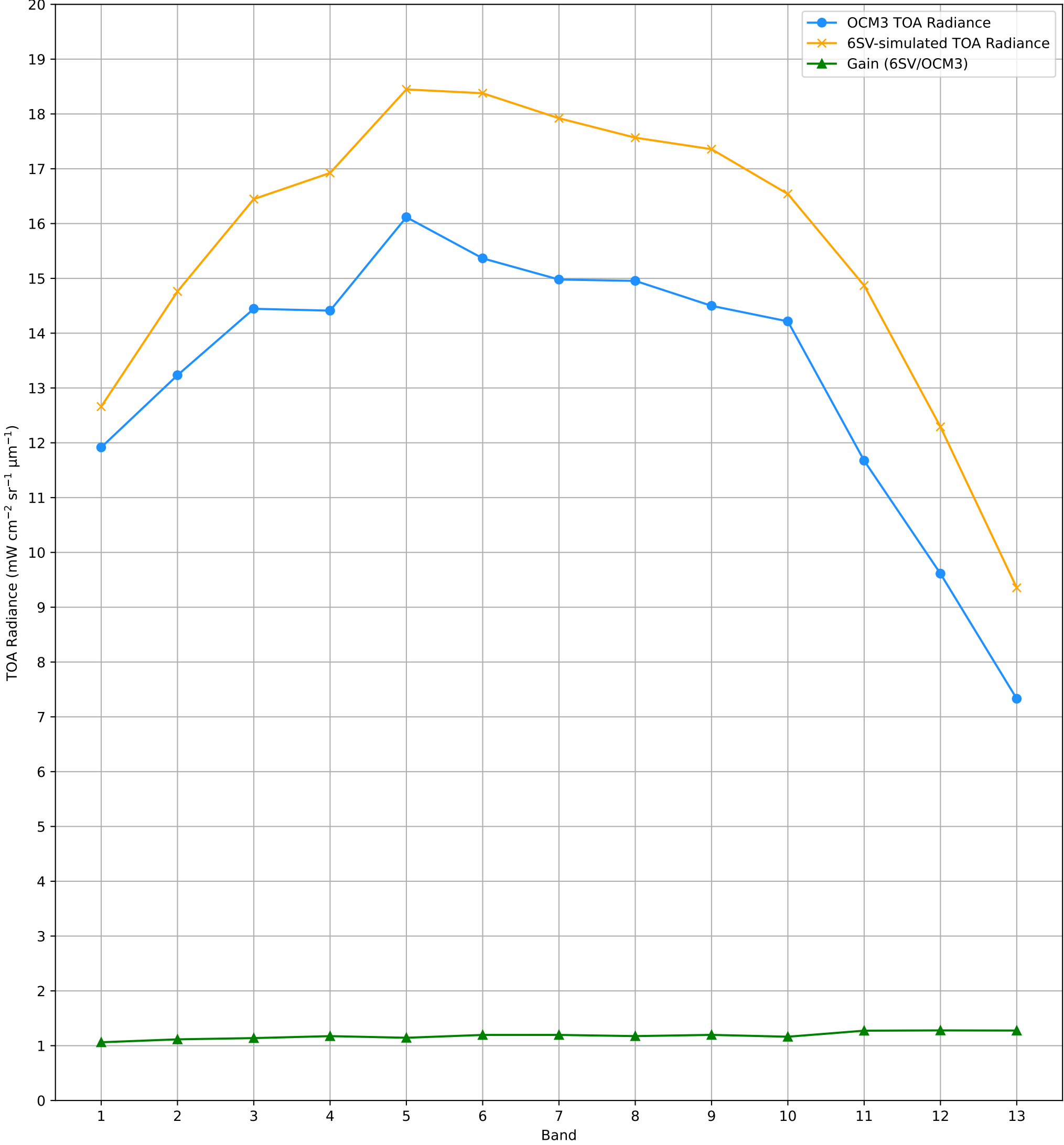
TOA Radiance (OCM3 vs. 6SV) over RVUS RadCalNet Site Lat: 38.497°, Lon: -115.69° - 10-JUL-2026 (STRIP_ID: 19127)
