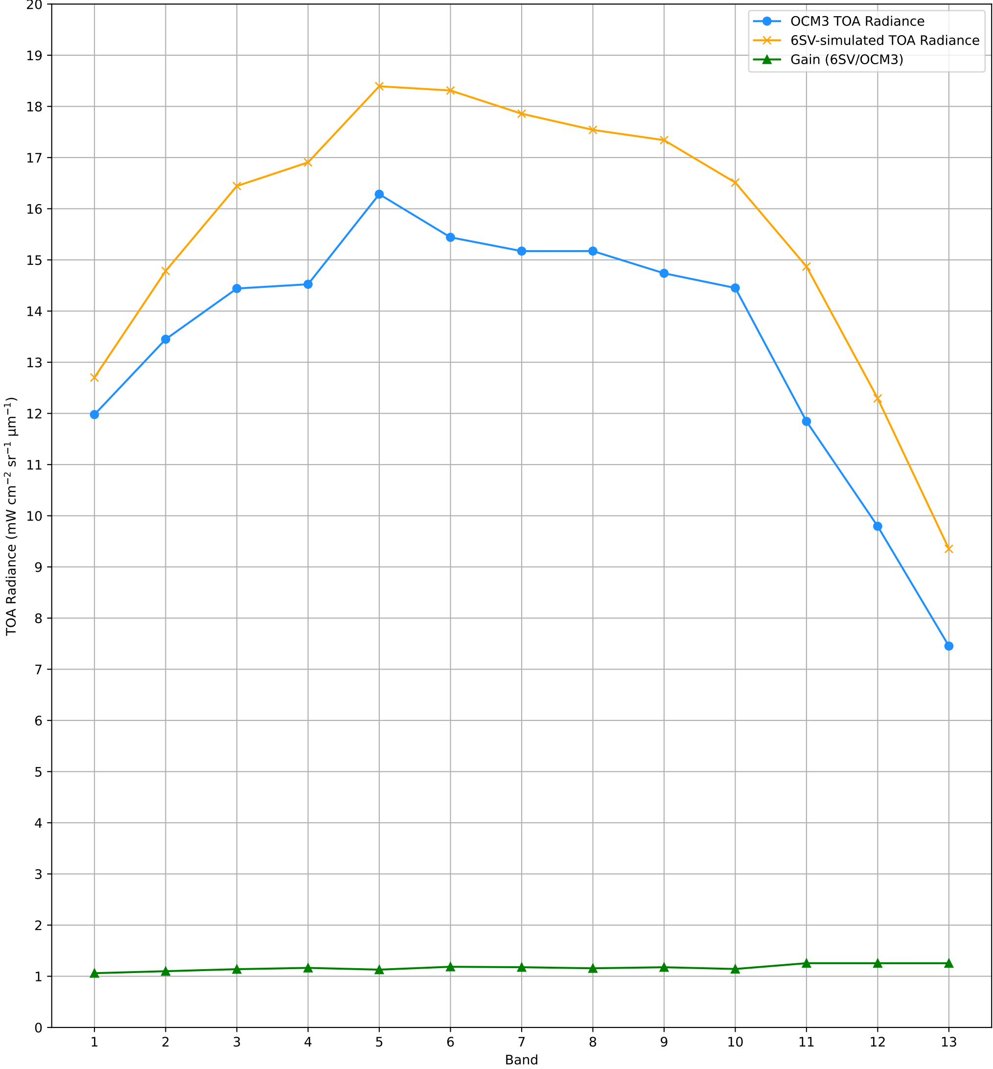
TOA Radiance (OCM3 vs. 6SV) over RVUS RadCalNet Site Lat: 38.497°, Lon: -115.69° - 08-JUL-2026 (STRIP_ID: 19098)
