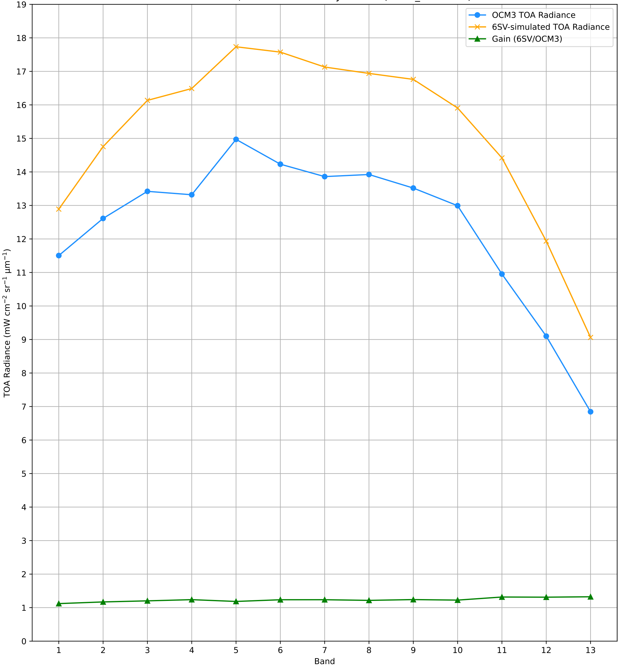
TOA Radiance (OCM3 vs. 6SV) over RVUS RadCalNet Site Lat: 38.497°, Lon: -115.69° - 07-JUL-2026 (STRIP_ID: 19084)
