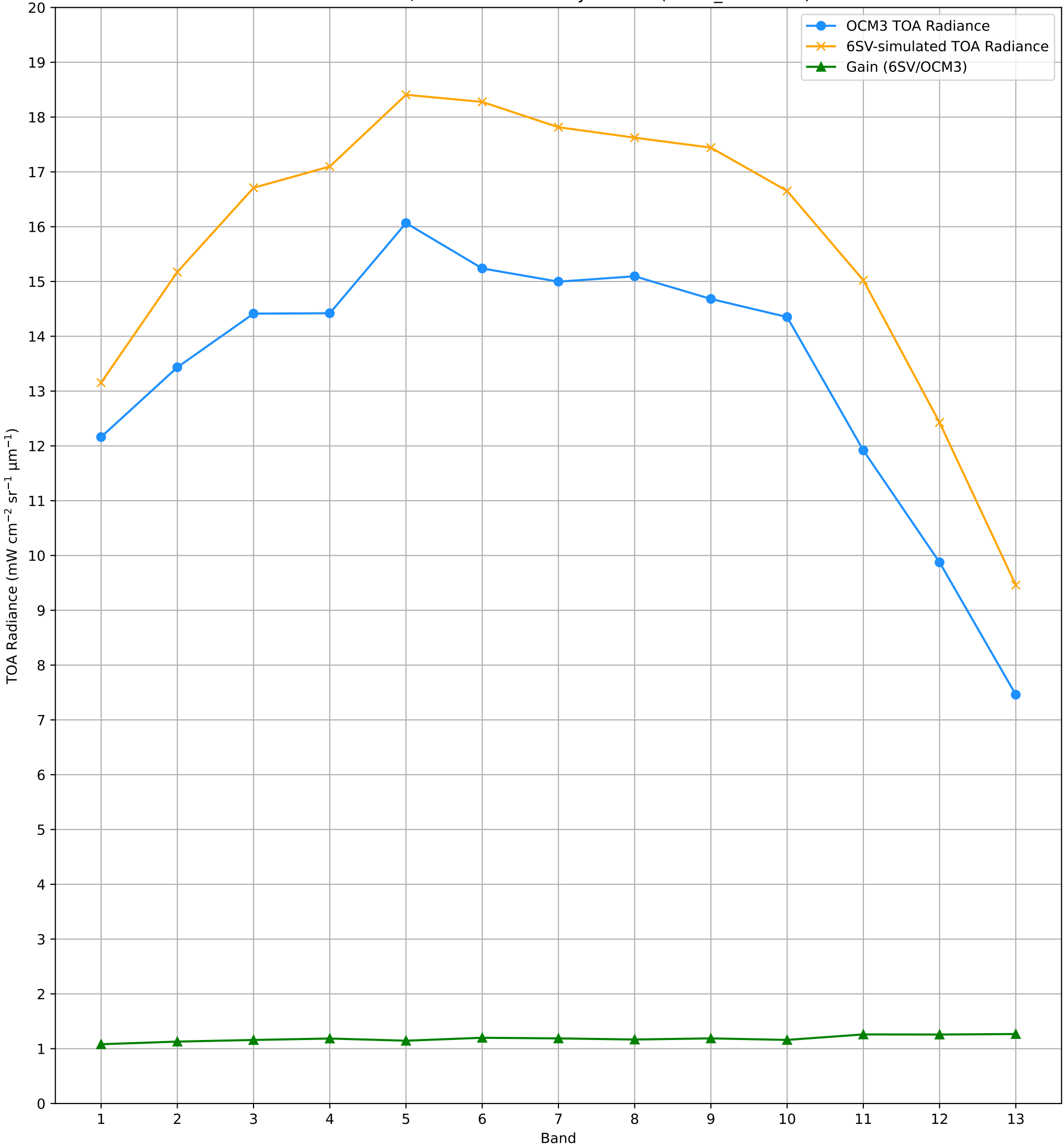
TOA Radiance (OCM3 vs. 6SV) over RVUS RadCalNet Site Lat: 38.497°, Lon: -115.69° - 04-JUL-2026 (STRIP_ID: 19040)
