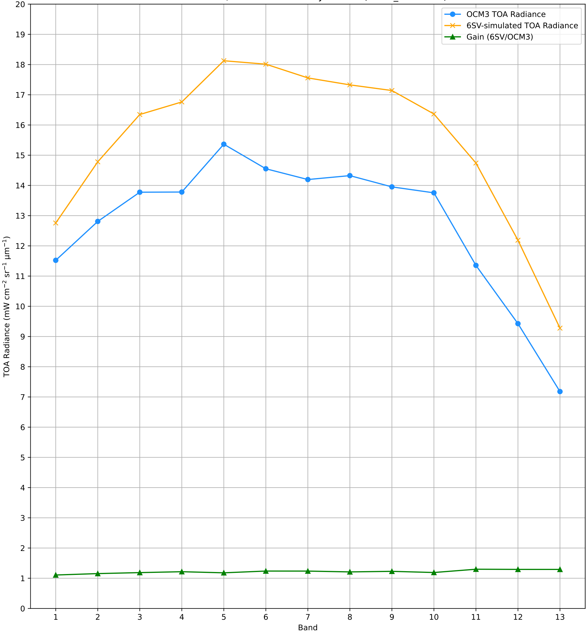
TOA Radiance (OCM3 vs. 6SV) over RVUS RadCalNet Site Lat: 38.497°, Lon: -115.69° - 03-JUL-2026 (STRIP_ID: 19026)
