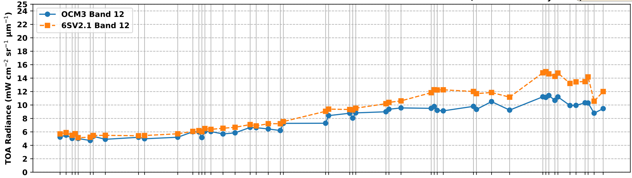
OCM3 Band 12 vs 6S Simulated Band 12 TOA Radiance over RVUS RadCalNet Site (Dec 2025 to May 2026)
