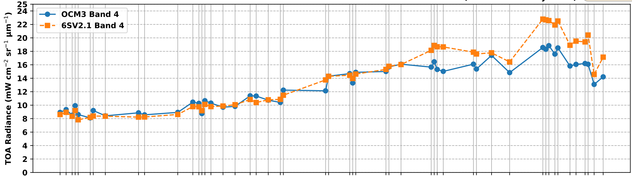
OCM3 Band 4 vs 6S Simulated Band 4 TOA Radiance over RVUS RadCalNet Site (Dec 2025 to May 2026)
