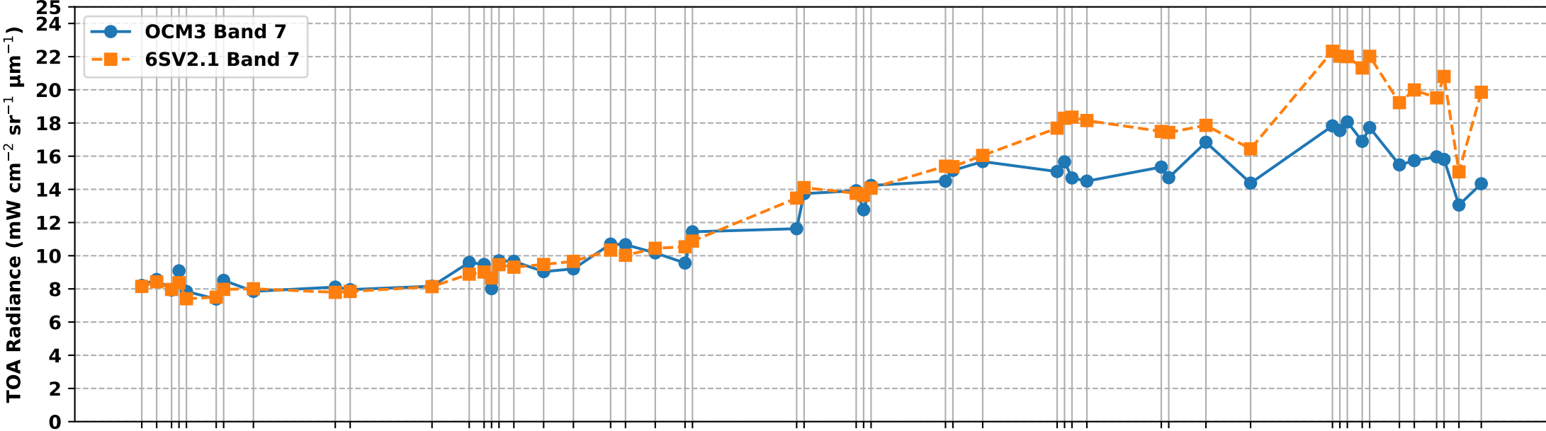
OCM3 Band 7 vs 6S Simulated Band 7 TOA Radiance over RVUS RadCalNet Site (Dec 2025 to May 2026)
