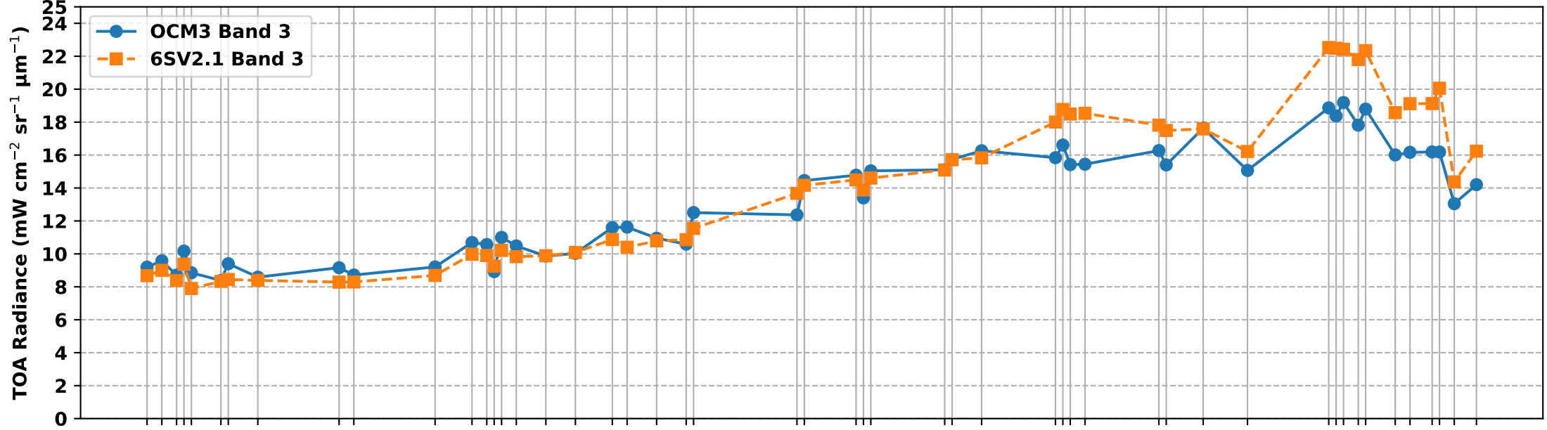
OCM3 Band 3 vs 6S Simulated Band 3 TOA Radiance over RVUS RadCalNet Site (Dec 2025 to May 2026)
