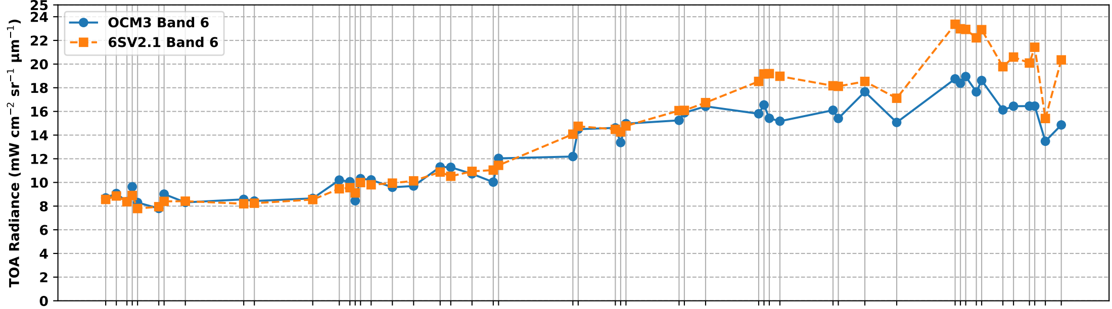
OCM3 Band 6 vs 6S Simulated Band 6 TOA Radiance over RVUS RadCalNet Site (Dec 2025 to May 2026)
