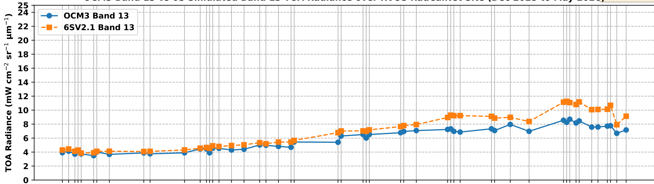
OCM3 Band 13 vs 6S Simulated Band 13 TOA Radiance over RVUS RadCalNet Site (Dec 2025 to May 2026)
