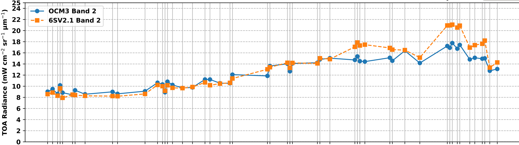
OCM3 Band 2 vs 6S Simulated Band 2 TOA Radiance over RVUS RadCalNet Site (Dec 2025 to May 2026)
