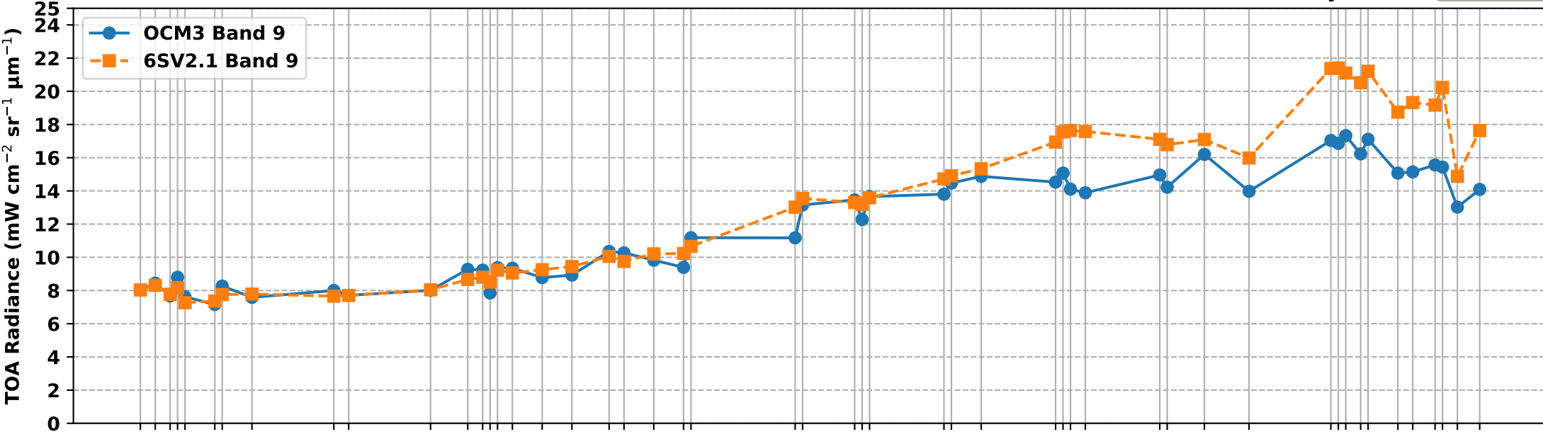
OCM3 Band 9 vs 6S Simulated Band 9 TOA Radiance over RVUS RadCalNet Site (Dec 2025 to May 2026)
