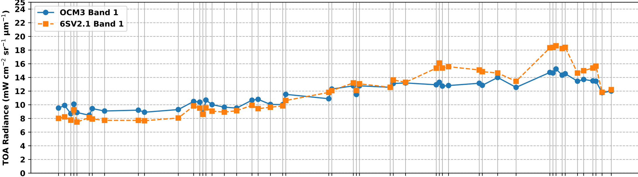
OCM3 Band 1 vs 6S Simulated Band 1 TOA Radiance over RVUS RadCalNet Site (Dec 2025 to May 2026)
