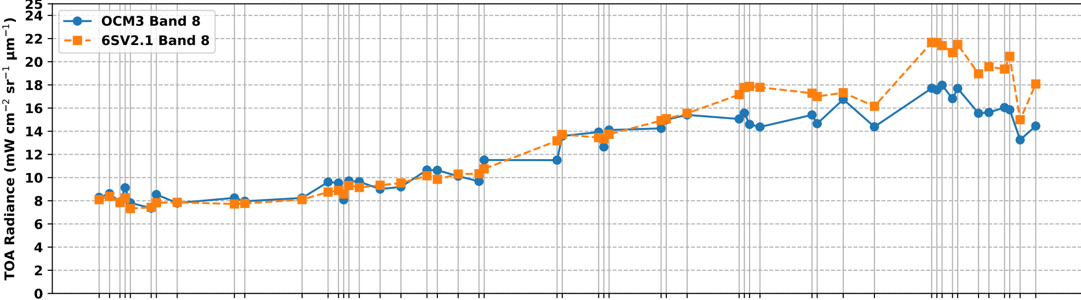
OCM3 Band 8 vs 6S Simulated Band 8 TOA Radiance over RVUS RadCalNet Site (Dec 2025 to May 2026)
