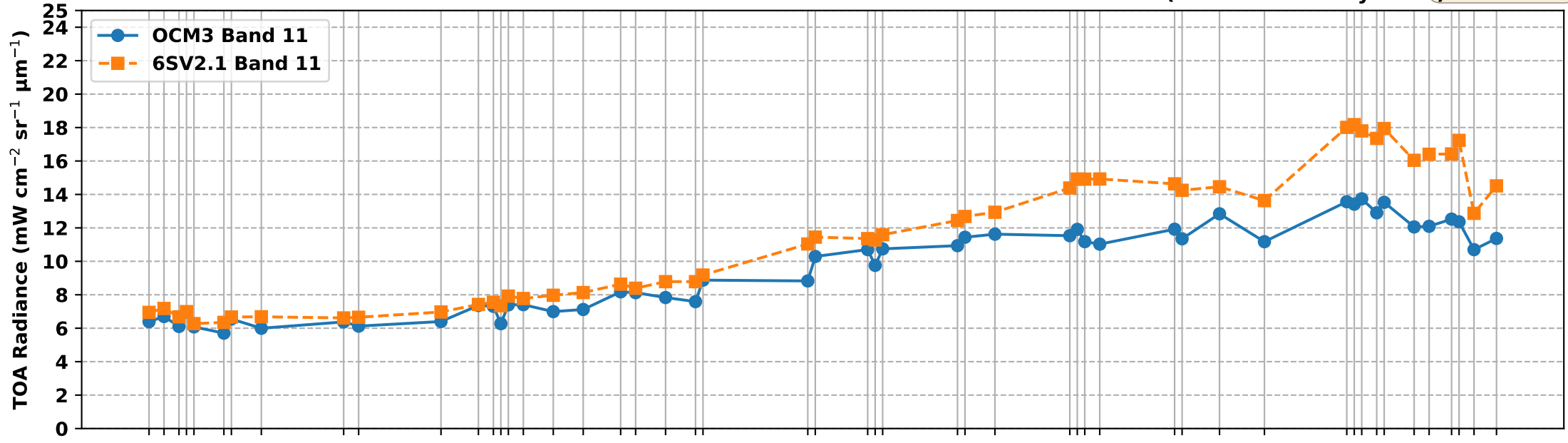
OCM3 Band 11 vs 6S Simulated Band 11 TOA Radiance over RVUS RadCalNet Site (Dec 2025 to May 2026)
