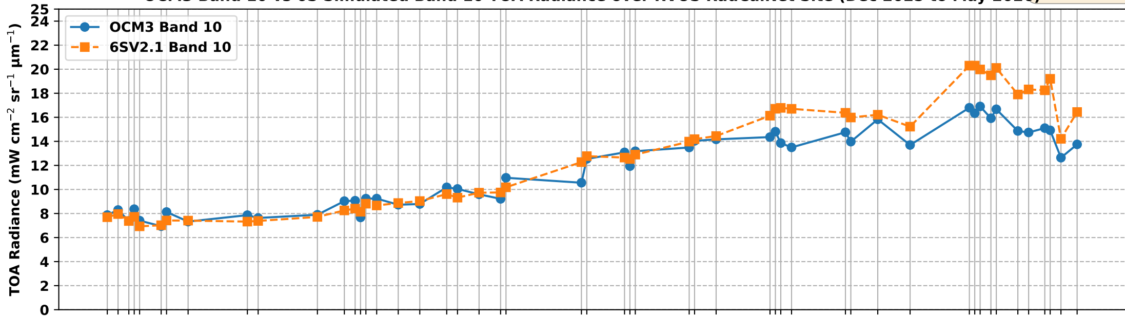
OCM3 Band 10 vs 6S Simulated Band 10 TOA Radiance over RVUS RadCalNet Site (Dec 2025 to May 2026)
