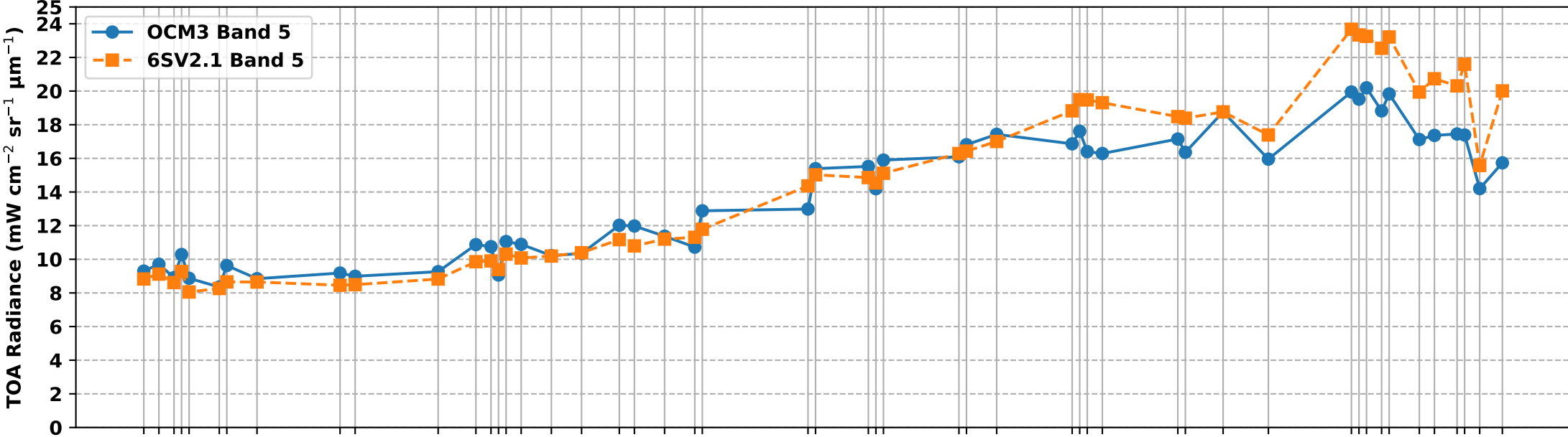
OCM3 Band 5 vs 6S Simulated Band 5 TOA Radiance over RVUS RadCalNet Site (Dec 2025 to May 2026)
