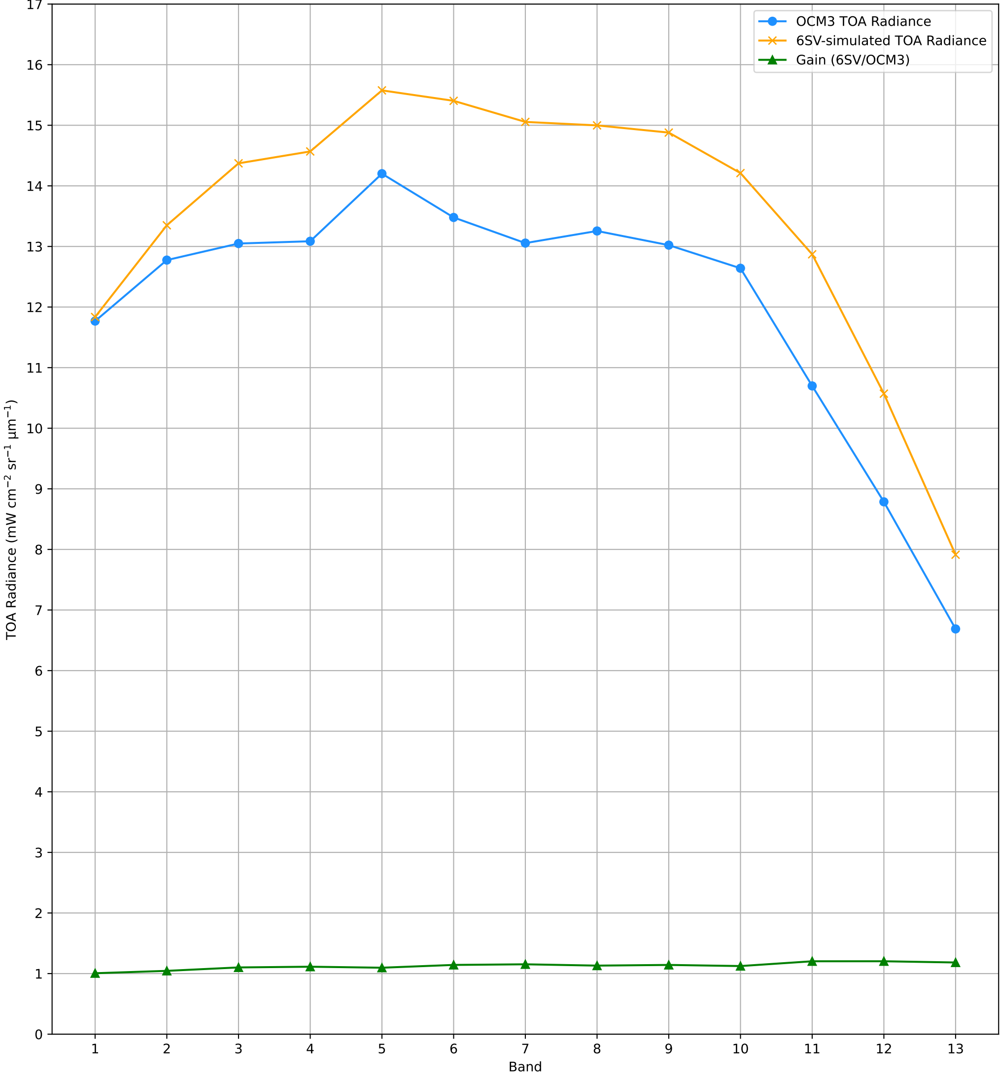
TOA Radiance (OCM3 vs. 6SV) over RVUS RadCalNet Site Lat: 38.497°, Lon: -115.69° - 27-MAY-2026 (STRIP_ID: 18491)
