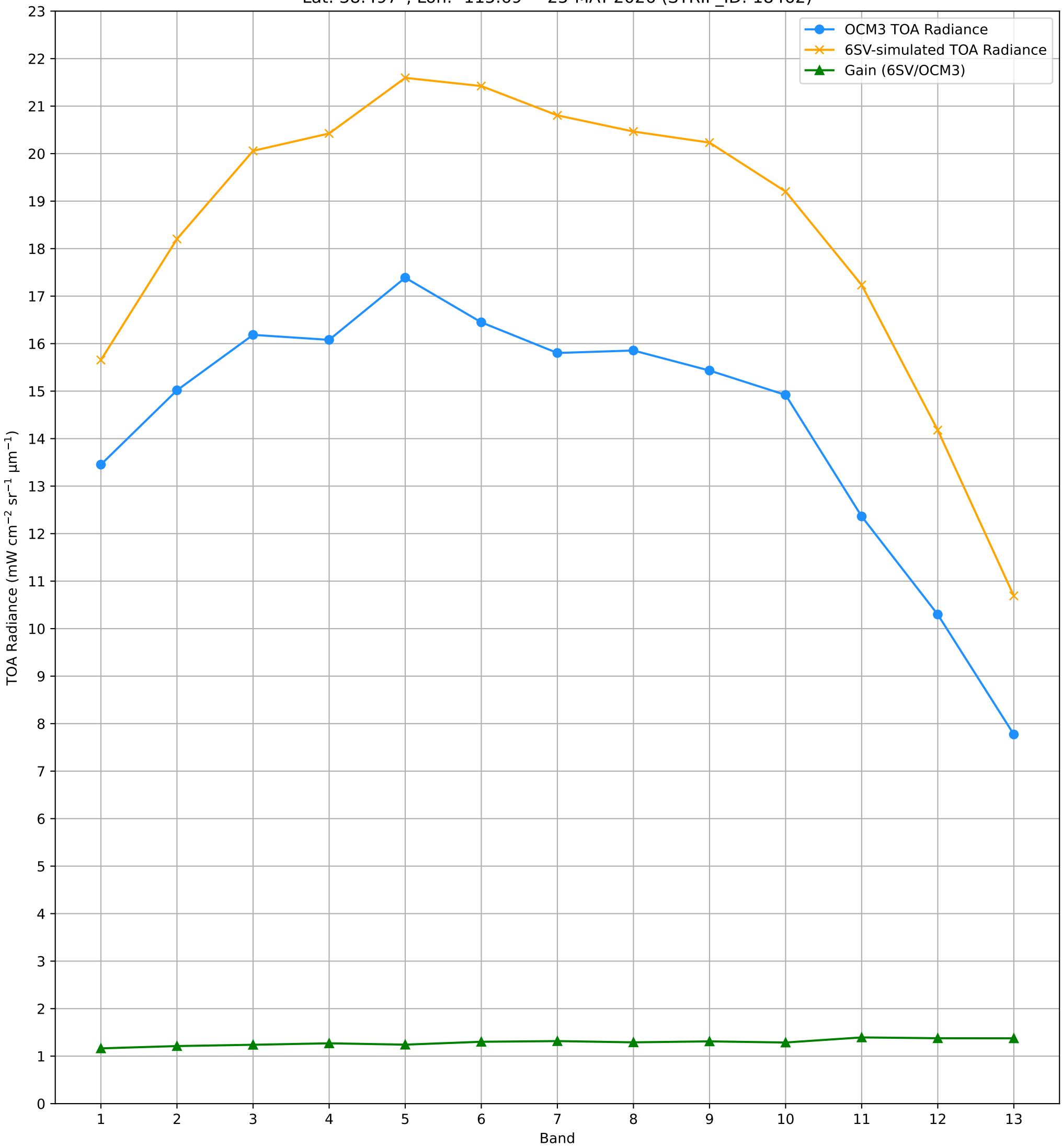
TOA Radiance (OCM3 vs. 6SV) over RVUS RadCalNet Site Lat: 38.497°, Lon: -115.69° - 25-MAY-2026 (STRIP_ID: 18462)
