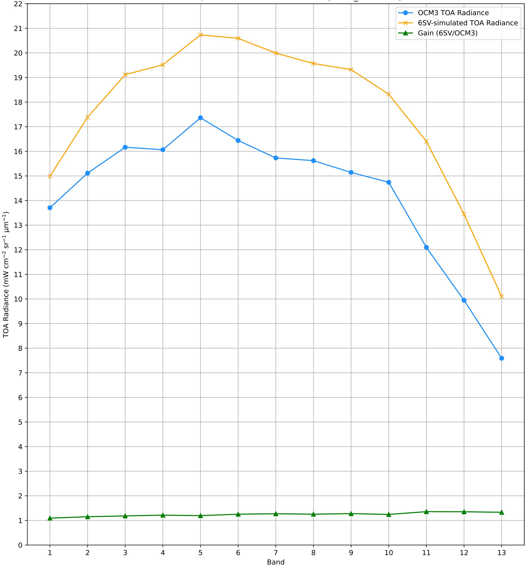
TOA Radiance (OCM3 vs. 6SV) over RVUS RadCalNet Site Lat: 38.497°, Lon: -115.69° - 21-MAY-2026 (STRIP_ID: 18404)
