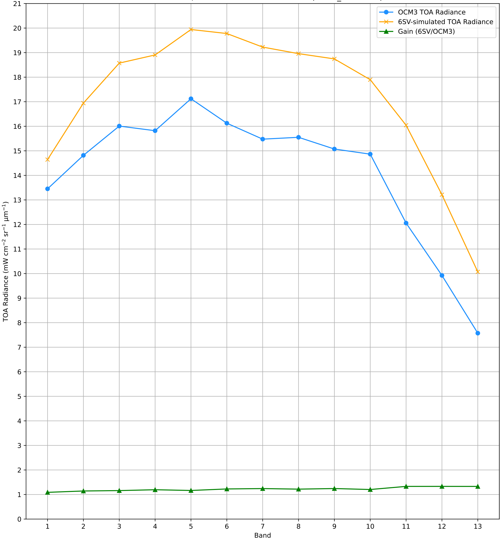
TOA Radiance (OCM3 vs. 6SV) over RVUS RadCalNet Site Lat: 38.497°, Lon: -115.69° - 19-MAY-2026 (STRIP_ID: 18375)
