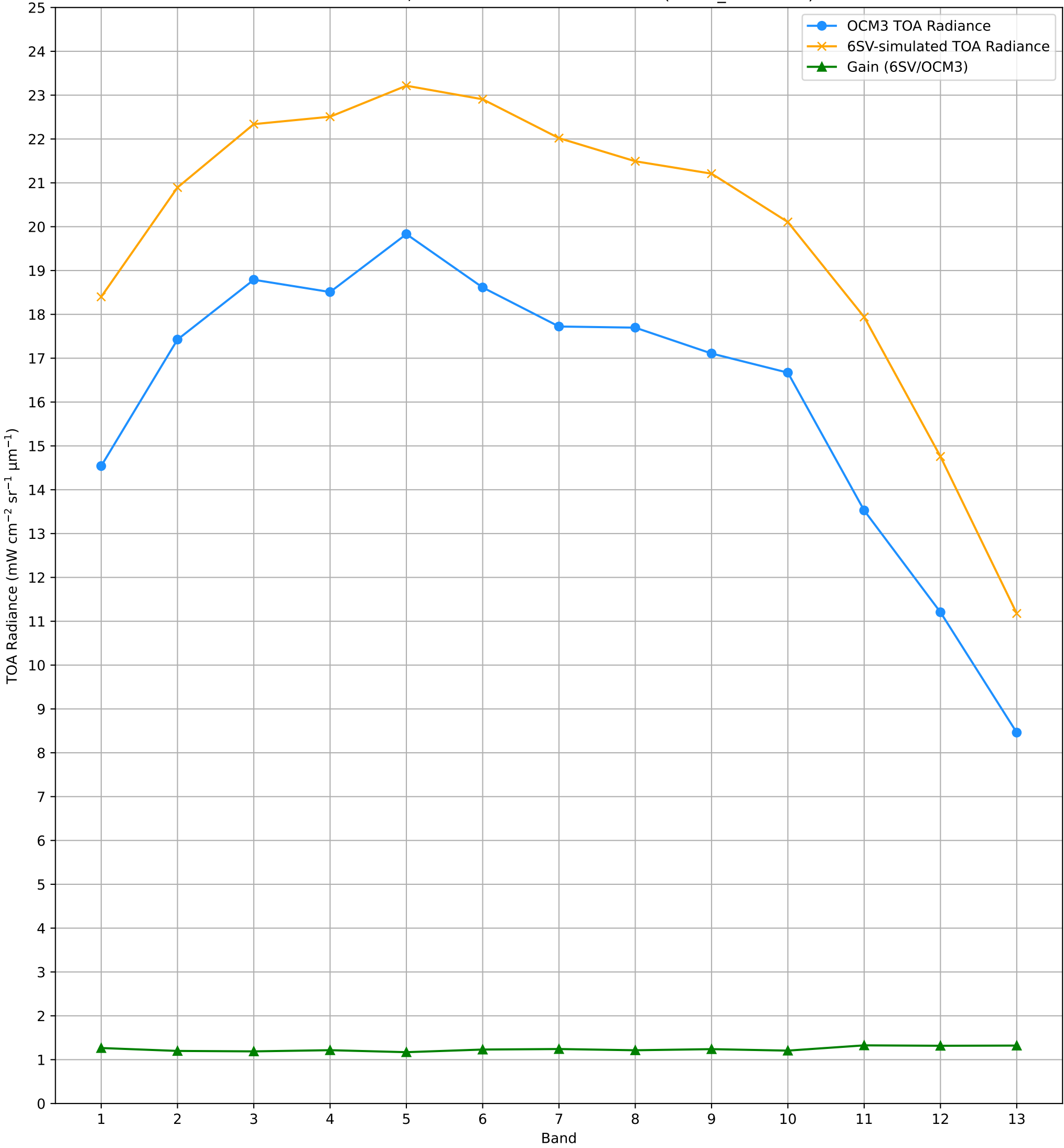
TOA Radiance (OCM3 vs. 6SV) over RVUS RadCalNet Site Lat: 38.497°, Lon: -115.69° - 15-MAY-2026 (STRIP_ID: 18317)
