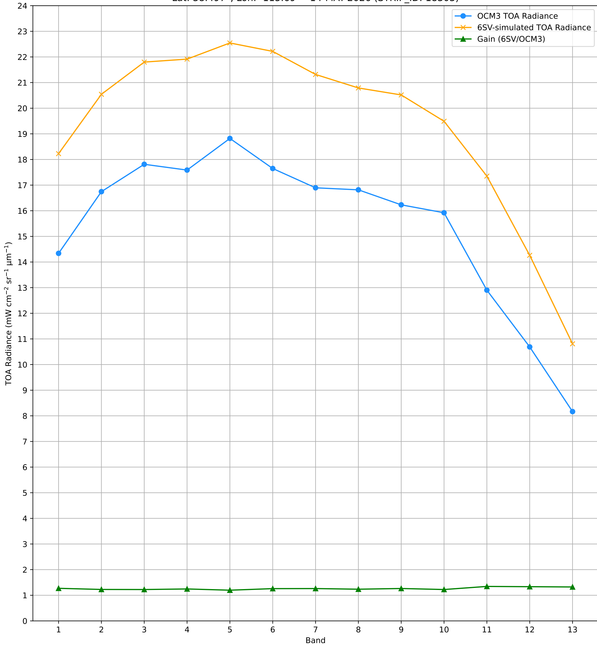
TOA Radiance (OCM3 vs. 6SV) over RVUS RadCalNet Site Lat: 38.497°, Lon: -115.69° - 14-MAY-2026 (STRIP_ID: 18303)
