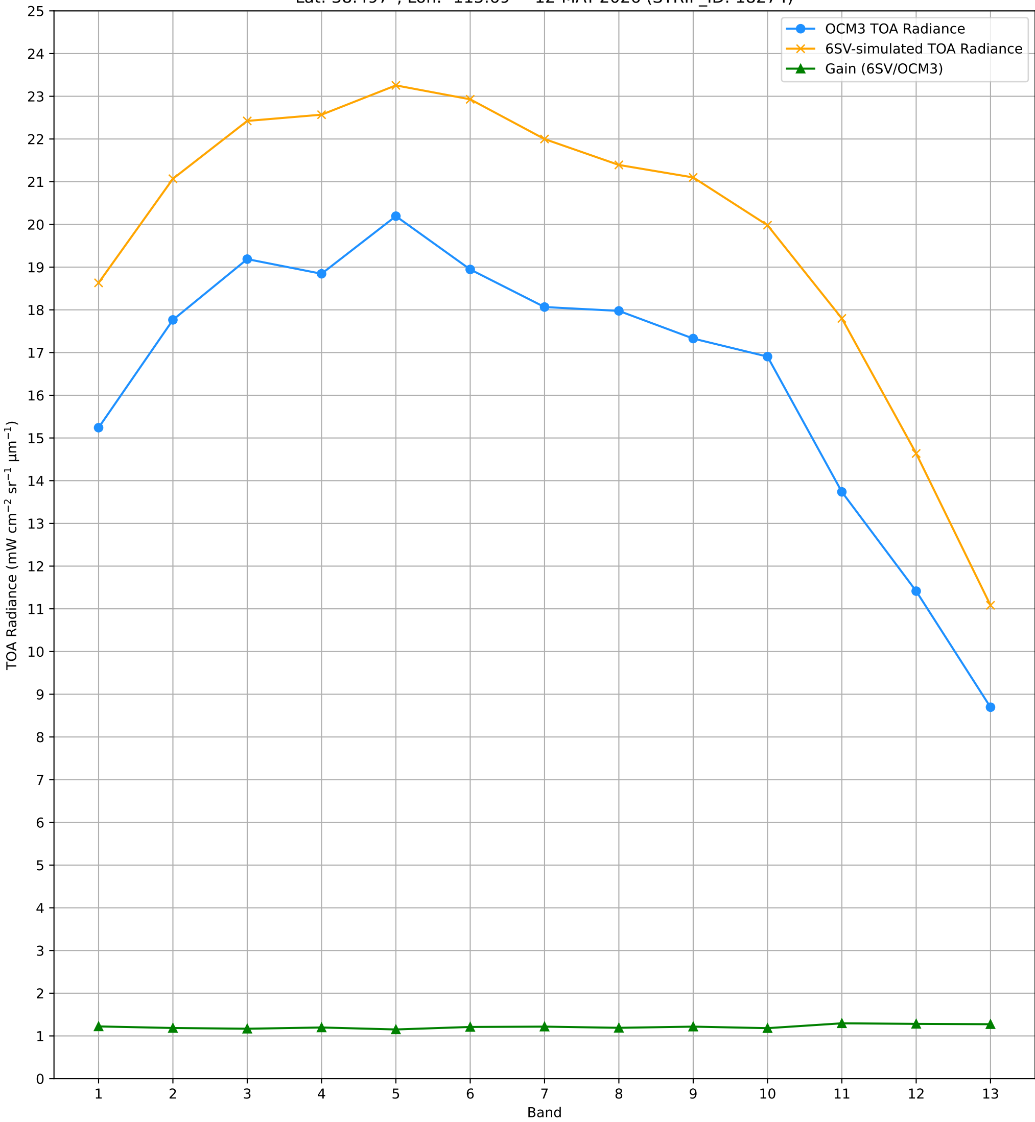
TOA Radiance (OCM3 vs. 6SV) over RVUS RadCalNet Site Lat: 38.497°, Lon: -115.69° - 12-MAY-2026 (STRIP_ID: 18274)
