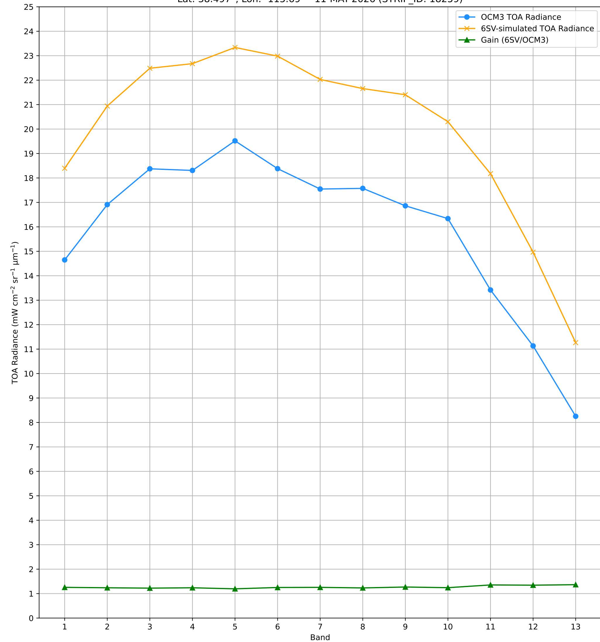
TOA Radiance (OCM3 vs. 6SV) over RVUS RadCalNet Site Lat: 38.497°, Lon: -115.69° - 11-MAY-2026 (STRIP_ID: 18259)
