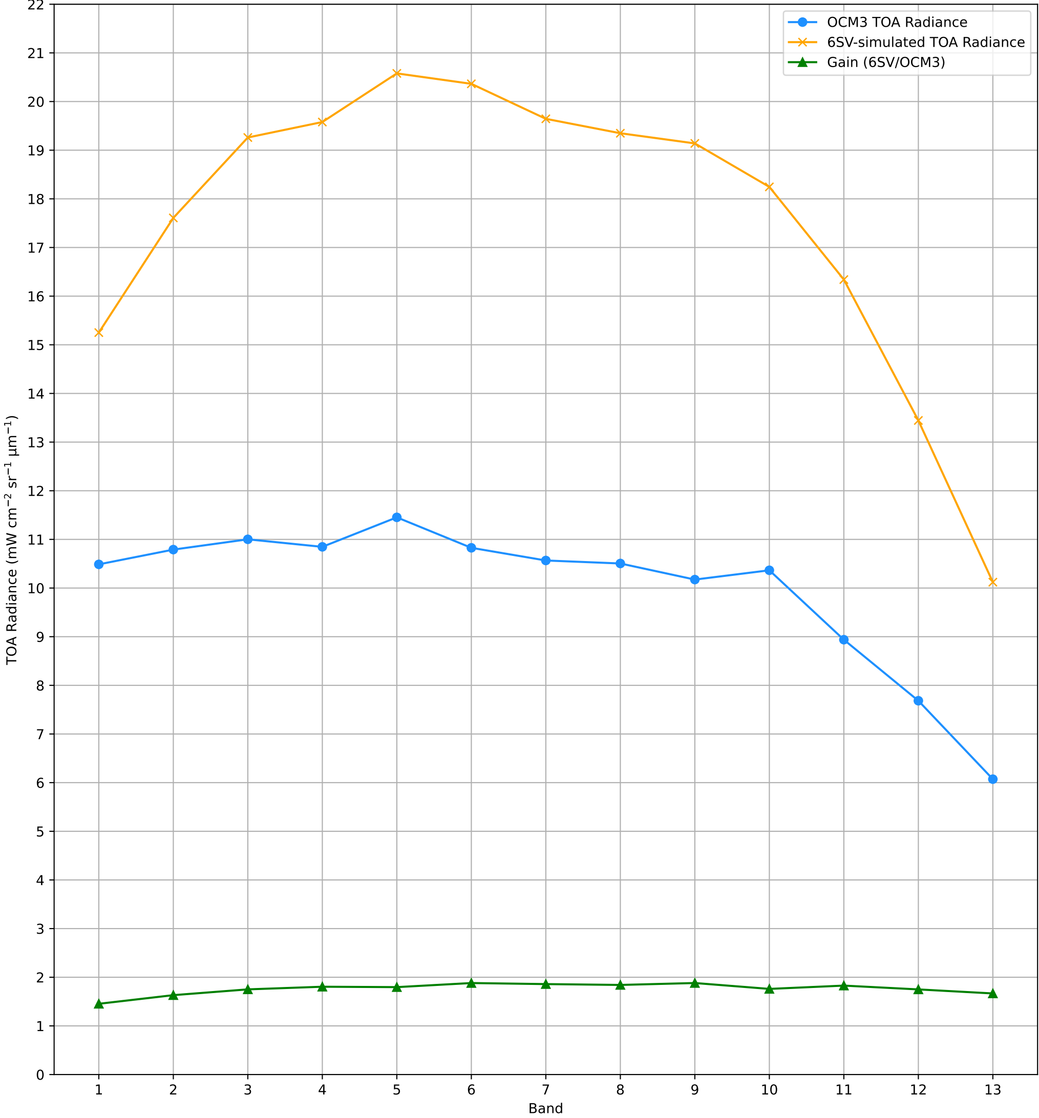
TOA Radiance (OCM3 vs. 6SV) over RVUS RadCalNet Site Lat: 38.497°, Lon: -115.69° - 22-JUN-2025 (STRIP_ID: 13588)
