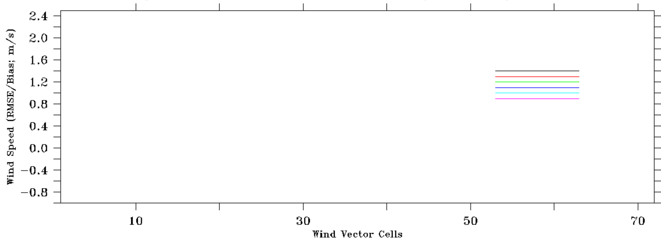
Comparison of SCATSAT-1 and NCMRWF for all passes over global oceans
