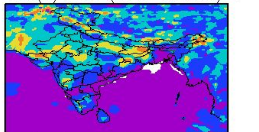
RH (%) RMSD (72 hr Forecast)
